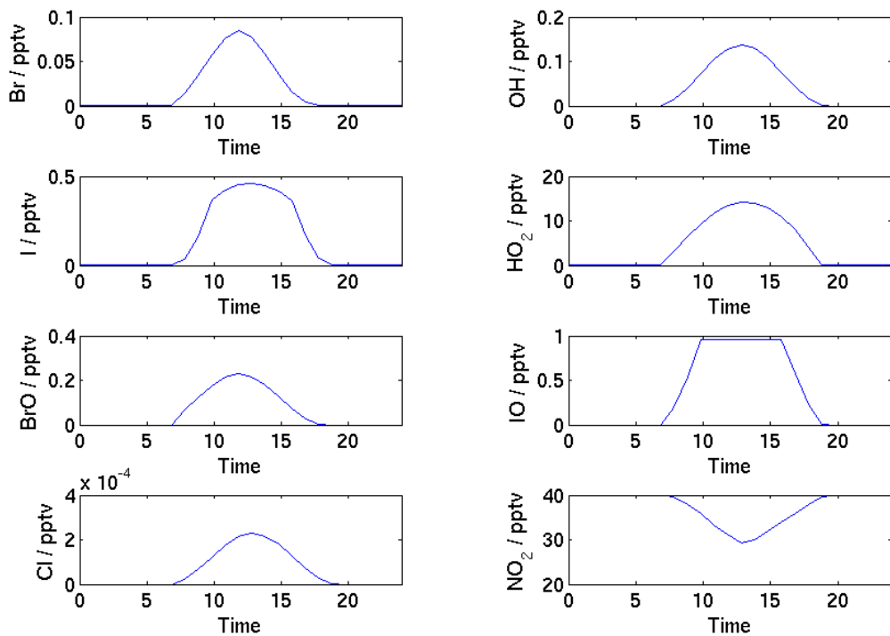
Fig. S1. Diurnal profiles of Br, BrO, I, IO, Cl, OH, HO 2 , and NO 2 used in the photochemical modelling for mercury oxidation.
