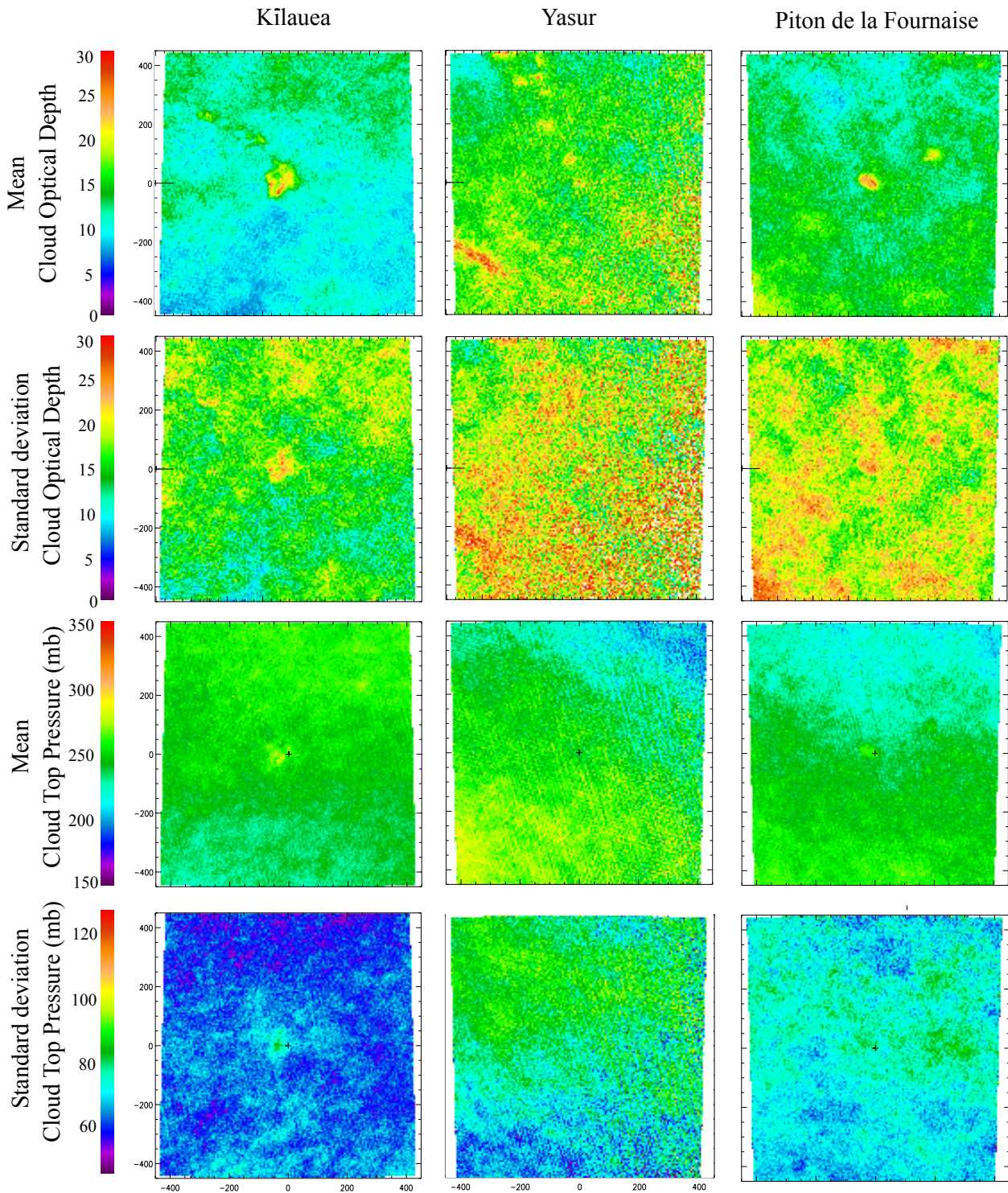
Multi-annual cloud property averages for MODIS (Aqua, MYDATML2) retrievals 2002-2013)
