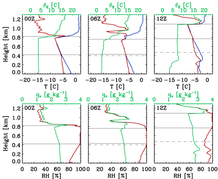
Fig. 4. Measurements from 0Z (left), 6Z (middle), and 12Z (right) soundings on 28 August 2008 (Case #1). Panels in the top row contain dry bulb (blue) and dew point (red) temperatures referenced to the lower axis and equivalent potential temperature (green) referenced to the upper axis. Panels in the lower row contain the relative humidity (red) referenced to the lower axis and specific humidity (green) referenced to the upper axis. In each panel, liquid cloud boundaries are designated by horizontal solid lines while the approximate base of the cloud-driven mixed layer is designated by a horizontal dashed line. Soundings are launched about 30 min prior to the nominal sounding time.
