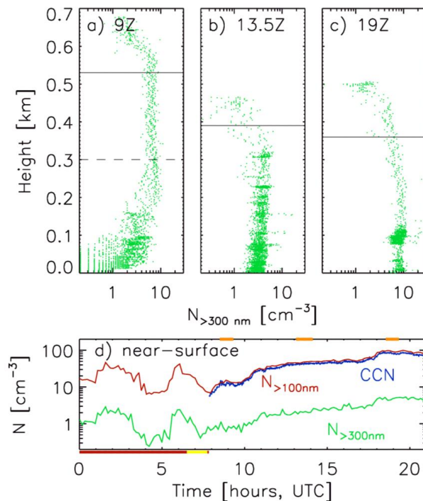
Fig. 8. Near-surface and helicopter aerosol measurements on 29 August 2008 (Case #2), including helicopter profiles of aerosol concentration for particles larger than 300 nm taken at about (a) 9Z, (b) 13.5Z, and (c) 19Z, and (d) concentrations of CCN (blue), aerosols larger than 100 nm (red) and aerosols larger than 300 nm (green) measured on board Oden . In (a–c), the solid and dashed lines are the cloud base and mixed-layer base heights determined by remote sensors at the time, respectively. Red and yellow bars on the lower axis of (d) indicate questionable data due to contamination, while the orange bars on the top axis show the times of the helicopter profiles.
