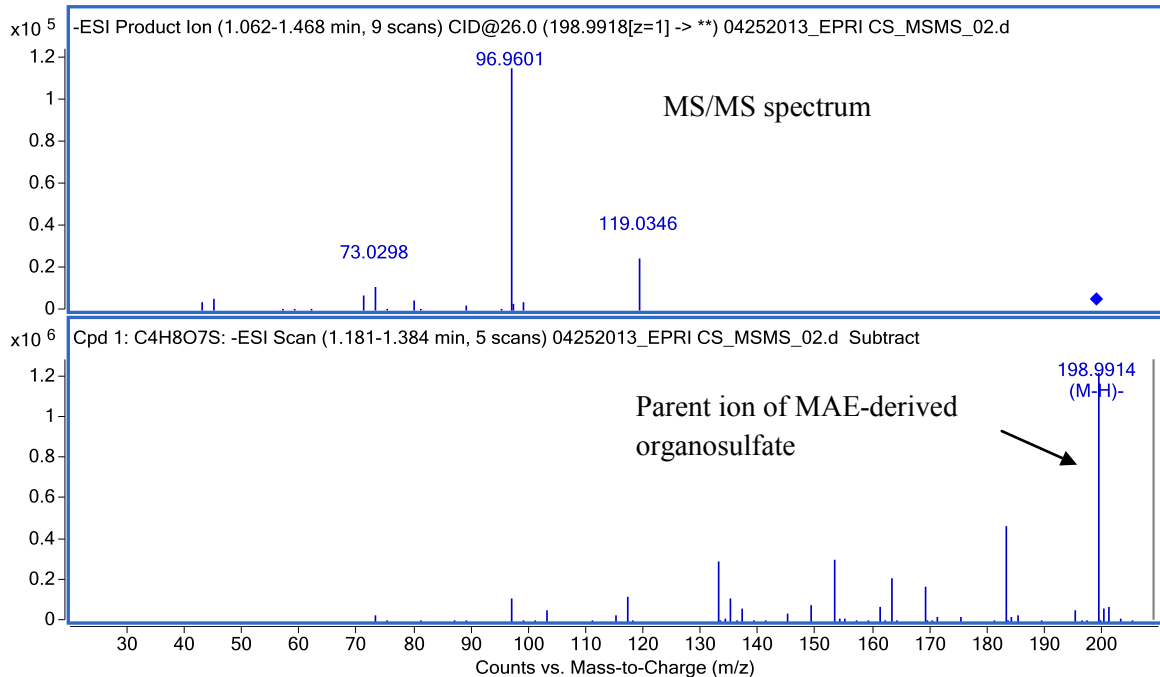
Fig. 1S. MS/MS spectrum of MAE-derived organosulfate (detected as the [M-H]^- ion at m/z 199).
