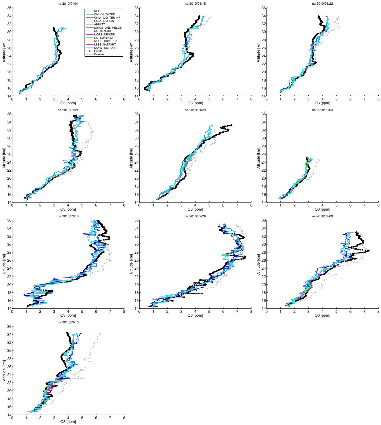
Figure 13: Measured ozone profiles (black dots) as a function of pressure altitude compared to modeled values of the reference run and all sensitivity runs (colored lines, color code in the first figure). The dashed grey line is the passive ozone profile.
