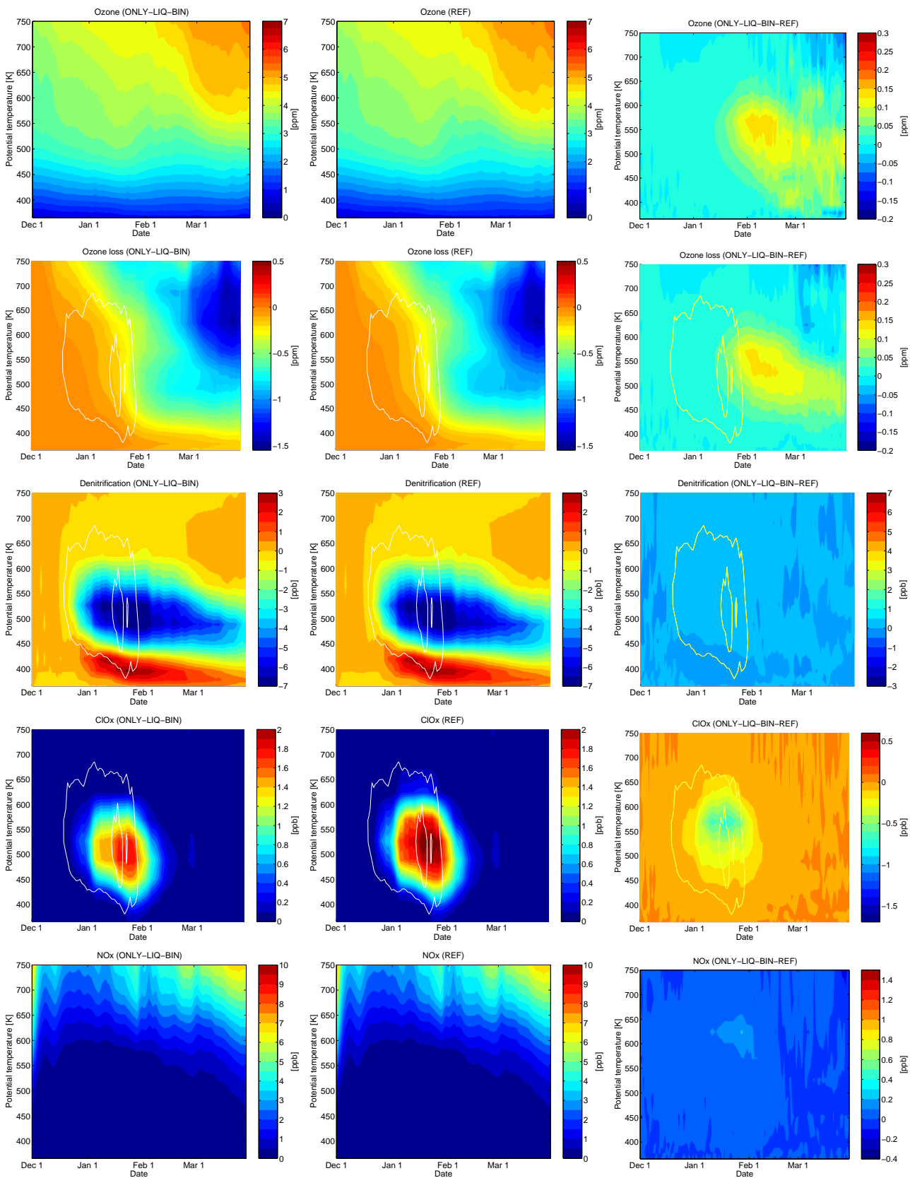
Figure 24: Vortex means as a function of model date and potential temperature inside the vortex boundary according to Nash. Left column: sensitivity run (ONLY-LIQ-BIN), middle column: reference run, right column: difference (sensitivity minus reference run). From top to bottom: ozone, ozone loss (difference of ozone to passive tracer), denitrification (difference of NO y to passive tracer), ClO x and NO x . White lines show the time periods where the formation of NAT clouds (outer line) and ice clouds (inner line) was possible inside the vortex.
