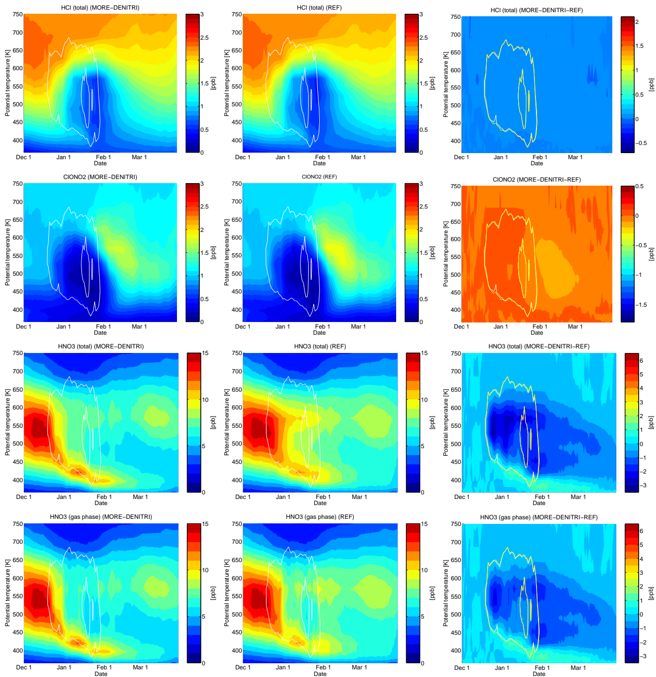
Figure 33: Vortex means as a function of model date and potential temperature inside the vortex boundary according to Nash. Left column: sensitivity run (MORE-DENITRI), middle column: reference run, right column: difference (sensitivity minus reference run). From top to bottom: HCl, ClONO 2 , HNO 3 (total), HNO 3 (gas phase). White lines show the time periods where the formation of NAT clouds (outer line) and ice clouds (inner line) was possible inside the vortex.
