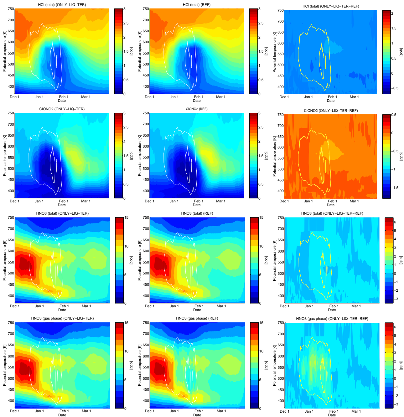
Figure 21: Vortex means as a function of model date and potential temperature inside the vortex boundary according to Nash. Left column: sensitivity run (ONLY-LIQ-TER), middle column: reference run, right column: difference (sensitivity minus reference run). From top to bottom: HCl, ClONO 2 , HNO 3 (total), HNO 3 (gas phase). White lines show the time periods where the formation of NAT clouds (outer line) and ice clouds (inner line) was possible inside the vortex.
