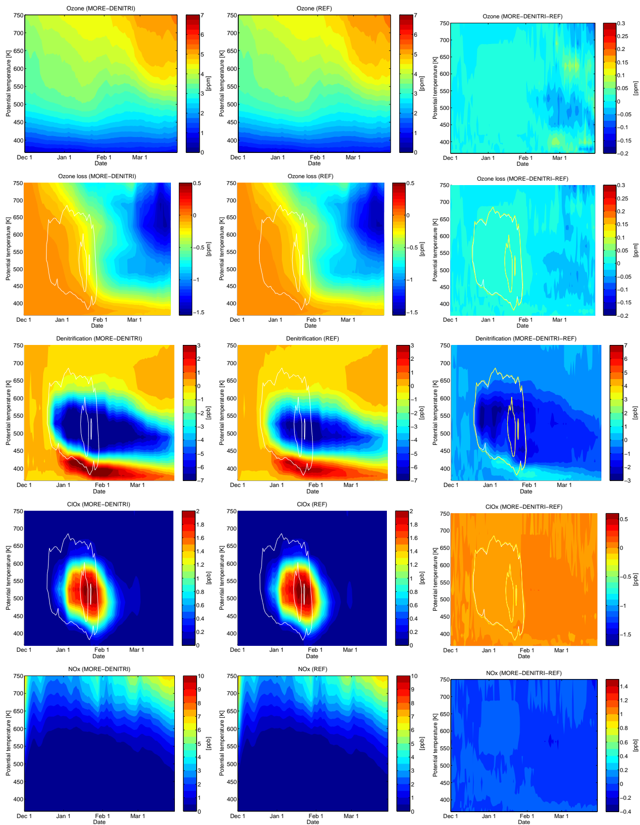
Figure 32: Vortex means as a function of model date and potential temperature inside the vortex boundary according to Nash. Left column: sensitivity run (MORE-DENITRI), middle column: reference run, right column: difference (sensitivity minus reference run). From top to bottom: ozone, ozone loss (difference of ozone to passive tracer), denitrification (difference of NO y to passive tracer), ClO x and NO x . White lines show the time periods where the formation of NAT clouds (outer line) and ice clouds (inner line) was possible inside the vortex.
