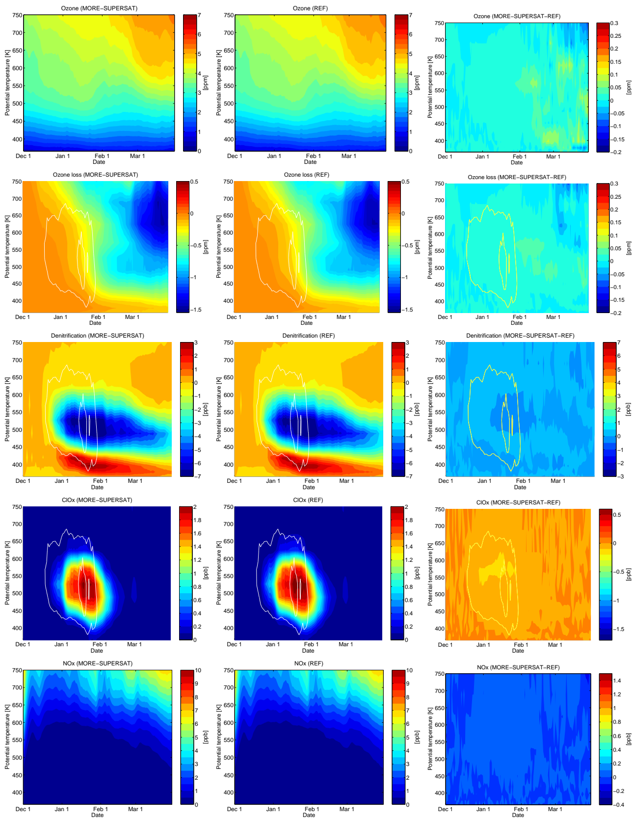
Figure 36: Vortex means as a function of model date and potential temperature inside the vortex boundary according to Nash. Left column: sensitivity run (MORE-SUPERSAT), middle column: reference run, right column: difference (sensitivity minus reference run). From top to bottom: ozone, ozone loss (difference of ozone to passive tracer), denitrification (difference of NO y to passive tracer), ClO x and NO x . White lines show the time periods where the formation of NAT clouds (outer line) and ice clouds (inner line) was possible inside the vortex.
