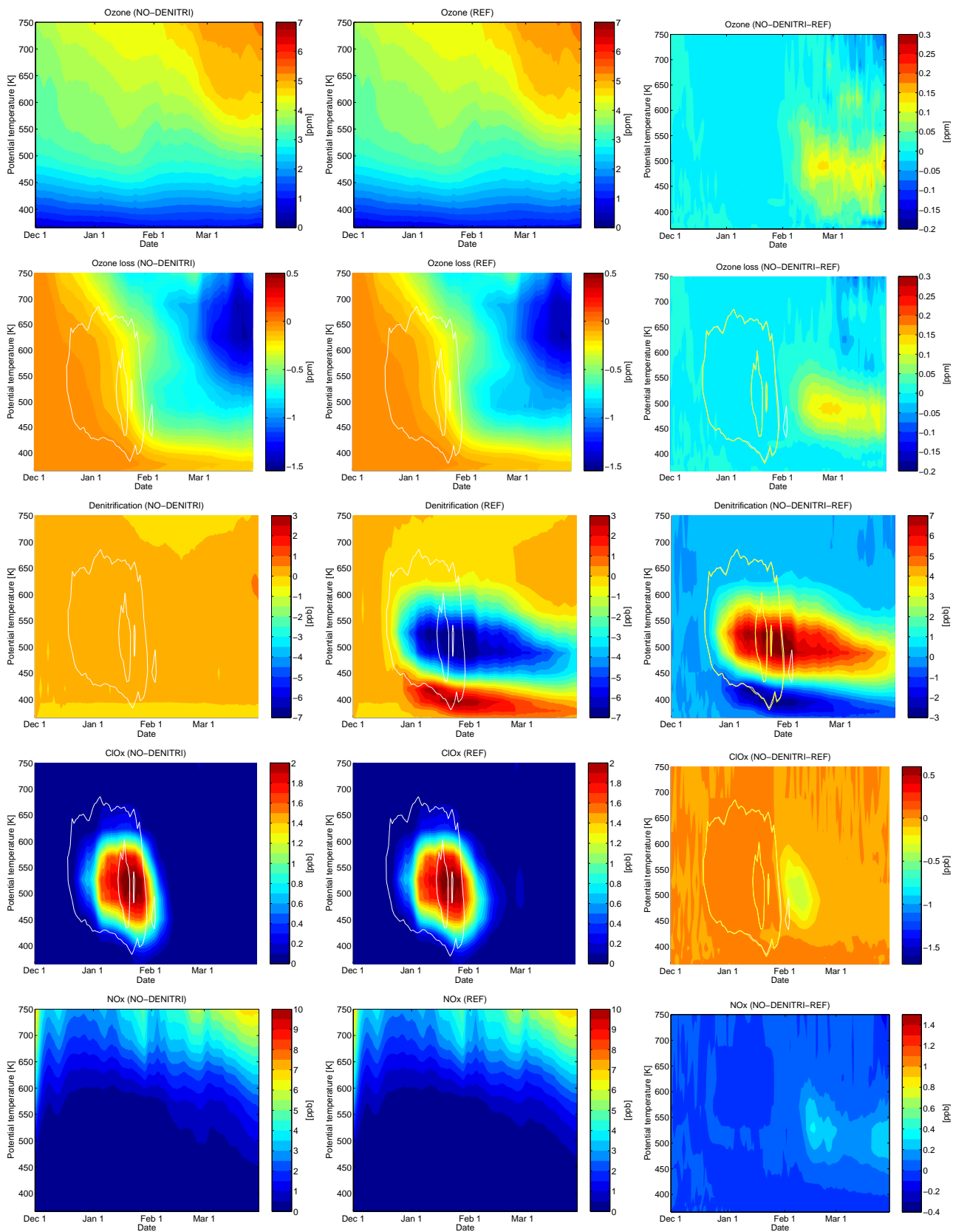
Figure 30: Vortex means as a function of model date and potential temperature inside the vortex boundary according to Nash. Left column: sensitivity run (NO-DENITRI), middle column: reference run, right column: difference (sensitivity minus reference run). From top to bottom: ozone, ozone loss (difference of ozone to passive tracer), denitrification (difference of \text{NO}_y to passive tracer), \text{ClO}_x and \text{NO}_x . White lines show the time periods where the formation of NAT clouds (outer line) and ice clouds (inner line) was possible inside the vortex.
