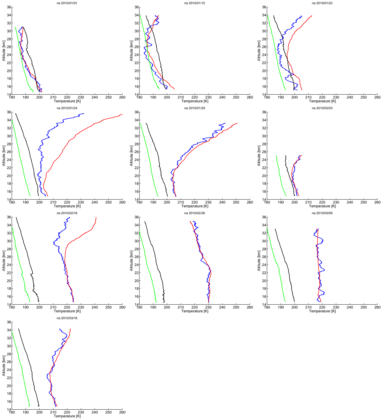
Figure 11: Temperature as a function of pressure altitude. The blue line shows the temperature measured by the sonde and the red line shows the temperature on the position of the probed air parcels at the last model time step before the flight (from the ERA Interim reanalysis). The thin black and green lines show the NAT and ice formation temperatures.
