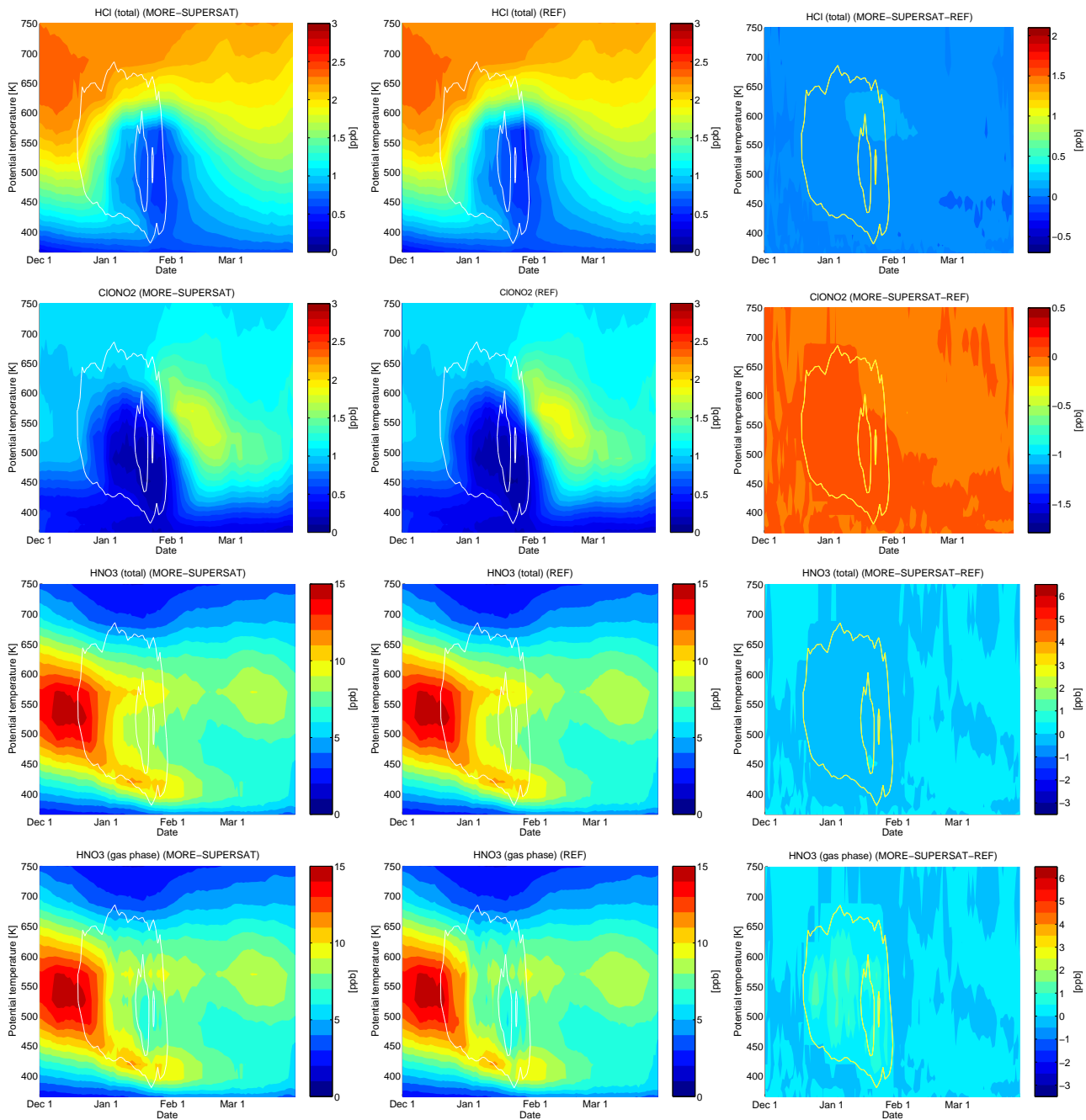
Figure 37: Vortex means as a function of model date and potential temperature inside the vortex boundary according to Nash. Left column: sensitivity run (MORE-SUPERSAT), middle column: reference run, right column: difference (sensitivity minus reference run). From top to bottom: HCl, ClONO 2 , HNO 3 (total), HNO 3 (gas phase). White lines show the time periods where the formation of NAT clouds (outer line) and ice clouds (inner line) was possible inside the vortex.
