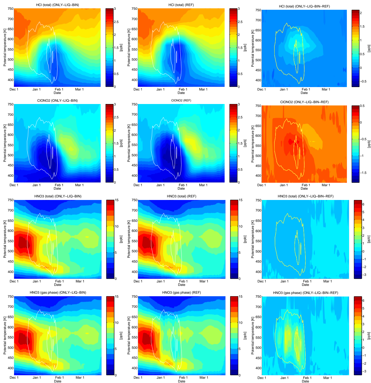
Figure 25: Vortex means as a function of model date and potential temperature inside the vortex boundary according to Nash. Left column: sensitivity run (ONLY-LIQ-BIN), middle column: reference run, right column: difference (sensitivity minus reference run). From top to bottom: HCl, ClONO 2 , HNO 3 (total), HNO 3 (gas phase). White lines show the time periods where the formation of NAT clouds (outer line) and ice clouds (inner line) was possible inside the vortex.
