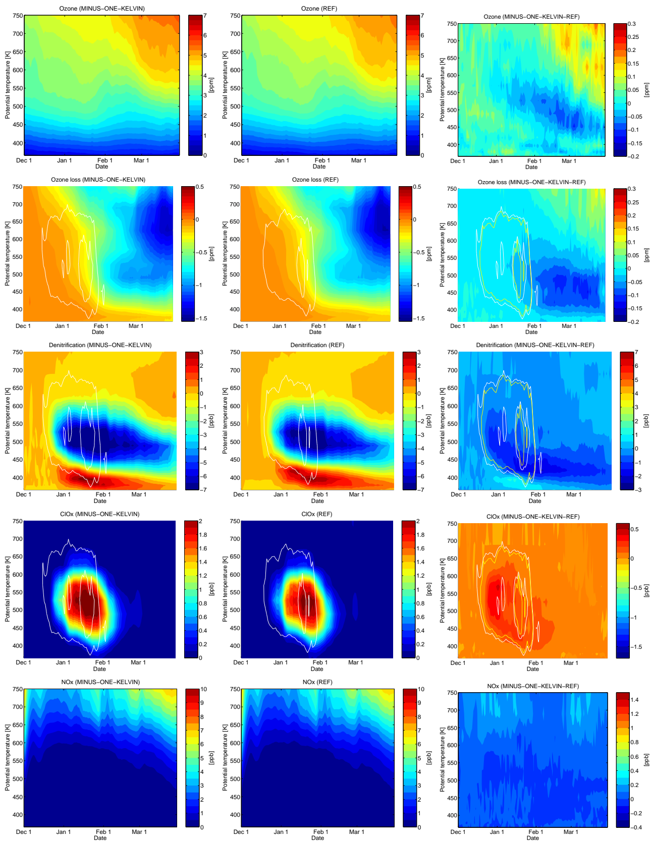
Figure 28: Vortex means as a function of model date and potential temperature inside the vortex boundary according to Nash. Left column: sensitivity run (MINUS-ONE-KELVIN), middle column: reference run, right column: difference (sensitivity minus reference run). From top to bottom: ozone, ozone loss (difference of ozone to passive tracer), denitrification (difference of NO y to passive tracer), ClO x and NO x . White lines show the time periods where the formation of NAT clouds (outer line) and ice clouds (inner line) was possible inside the vortex.
