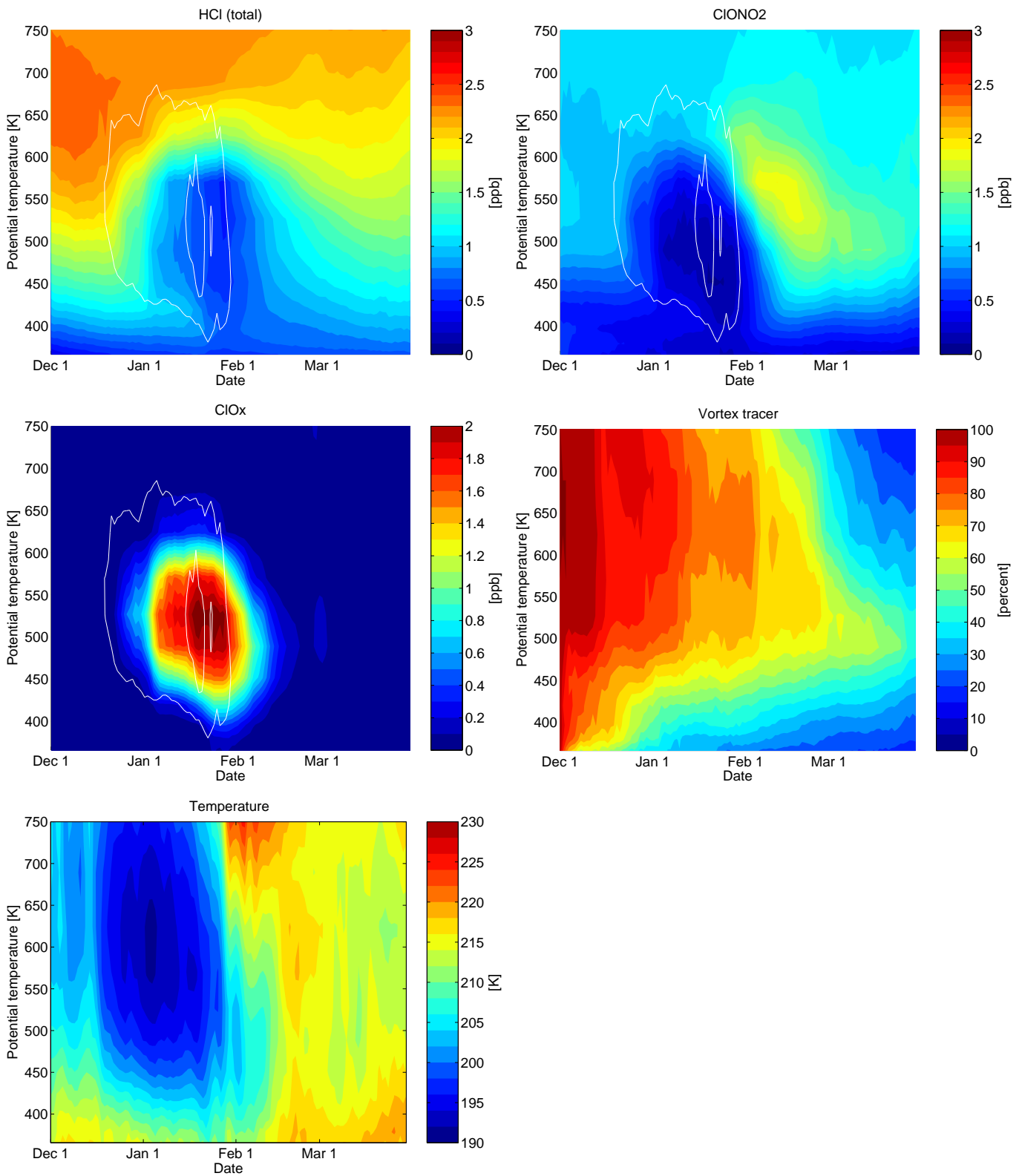
Figure 19: Vortex means as a function of model date and potential temperature inside the vortex boundary according to Nash. HCl, ClONO 2 , ClO x , vortex tracer, temperature. White lines show the time periods where the formation of NAT clouds (outer line) and ice clouds (inner line) was possible inside the vortex. One of the plots shows an approximate tracer for the vortex (initialized on 1 December with values of 100% inside 64° equivalent latitude and 0% elsewhere).
