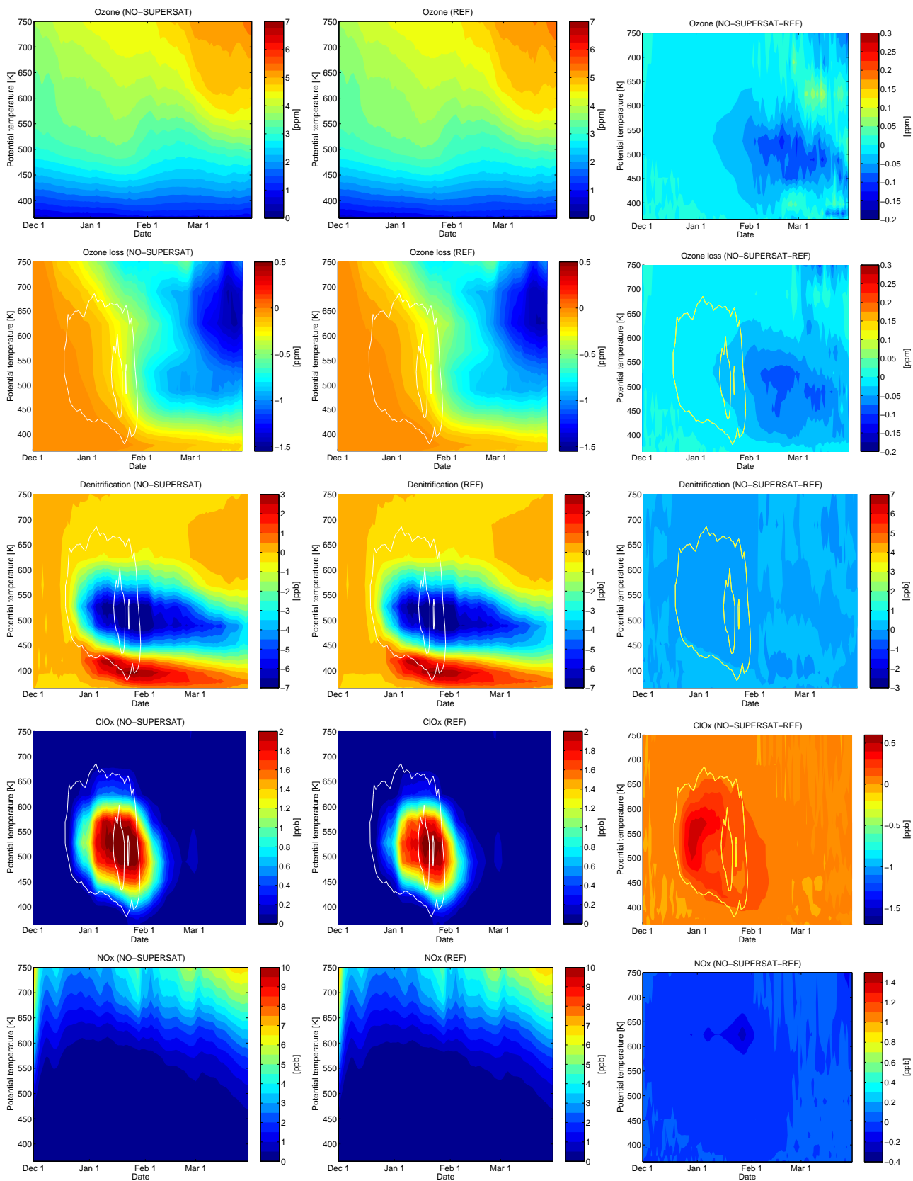
Figure 34: Vortex means as a function of model date and potential temperature inside the vortex boundary according to Nash. Left column: sensitivity run (NO-SUPERSAT), middle column: reference run, right column: difference (sensitivity minus reference run). From top to bottom: ozone, ozone loss (difference of ozone to passive tracer), denitrification (difference of NO y to passive tracer), ClO x and NO x . White lines show the time periods where the formation of NAT clouds (outer line) and ice clouds (inner line) was possible inside the vortex.
