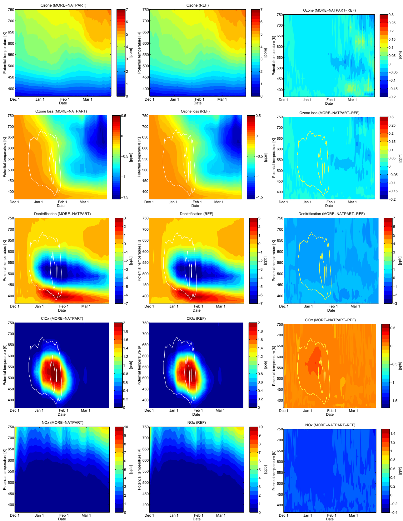
Figure 40: Vortex means as a function of model date and potential temperature inside the vortex boundary according to Nash. Left column: sensitivity run (MORE-NATPART), middle column: reference run, right column: difference (sensitivity minus reference run). From top to bottom: ozone, ozone loss (difference of ozone to passive tracer), denitrification (difference of NO y to passive tracer), ClO x and NO x . White lines show the time periods where the formation of NAT clouds (outer line) and ice clouds (inner line) was possible inside the vortex.
