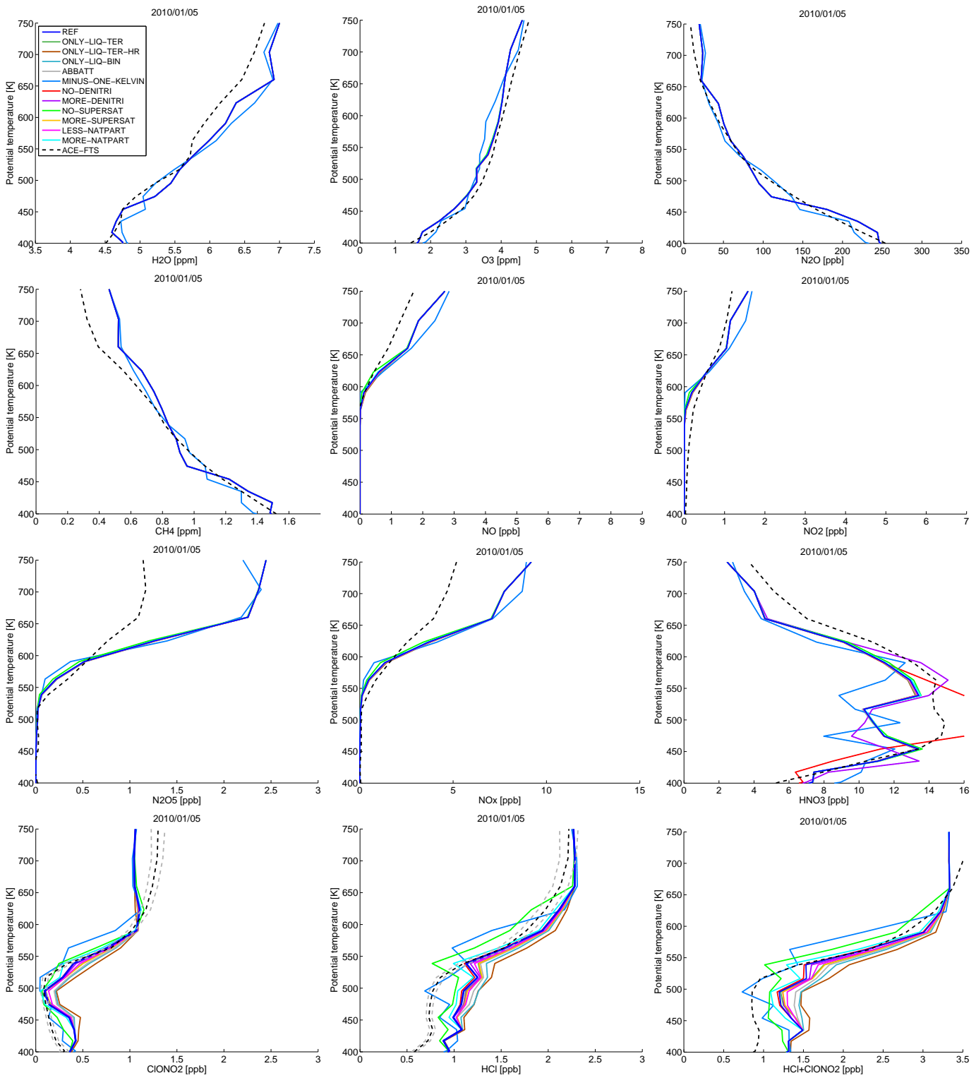
Figure 14: Example measurements of ACE-FTS on 5 January (56.8° N, 15.1° E) inside the vortex (black dashed lines). Profiles of H 2 O, O 3 , N 2 O, CH 4 , NO, NO 2 , N 2 O 5 , NO x = NO + NO 2 + 2N 2 O 5 , HNO 3 (gas phase), ClONO 2 , HCl and HCl + ClONO 2 . Colored lines show sensitivity runs (color code in the first figure).
