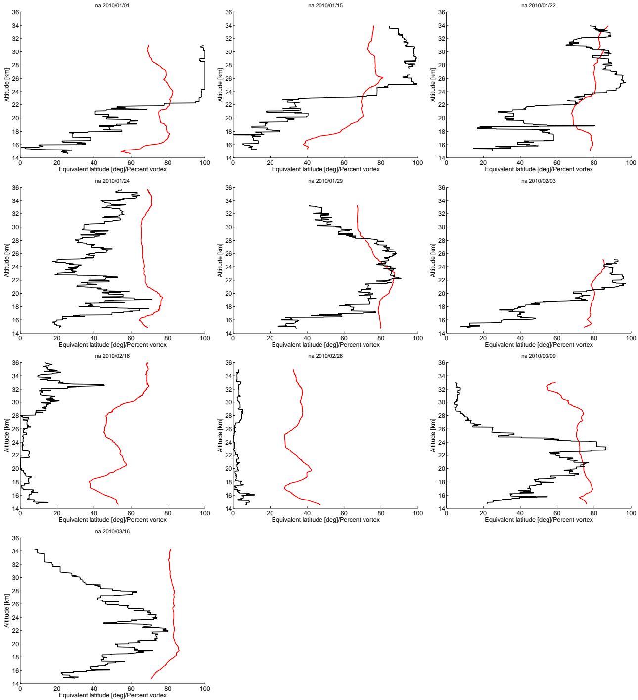
Figure 12: Equivalent latitude (red) as a function of pressure altitude calculated on the position of the probed air parcels at the last model time step before the flight from potential vorticity fields of the ERA Interim reanalysis. The black line shows an approximate tracer for the vortex (initialized on 1 December with values of 100% inside 64° equivalent latitude and 0% elsewhere).
