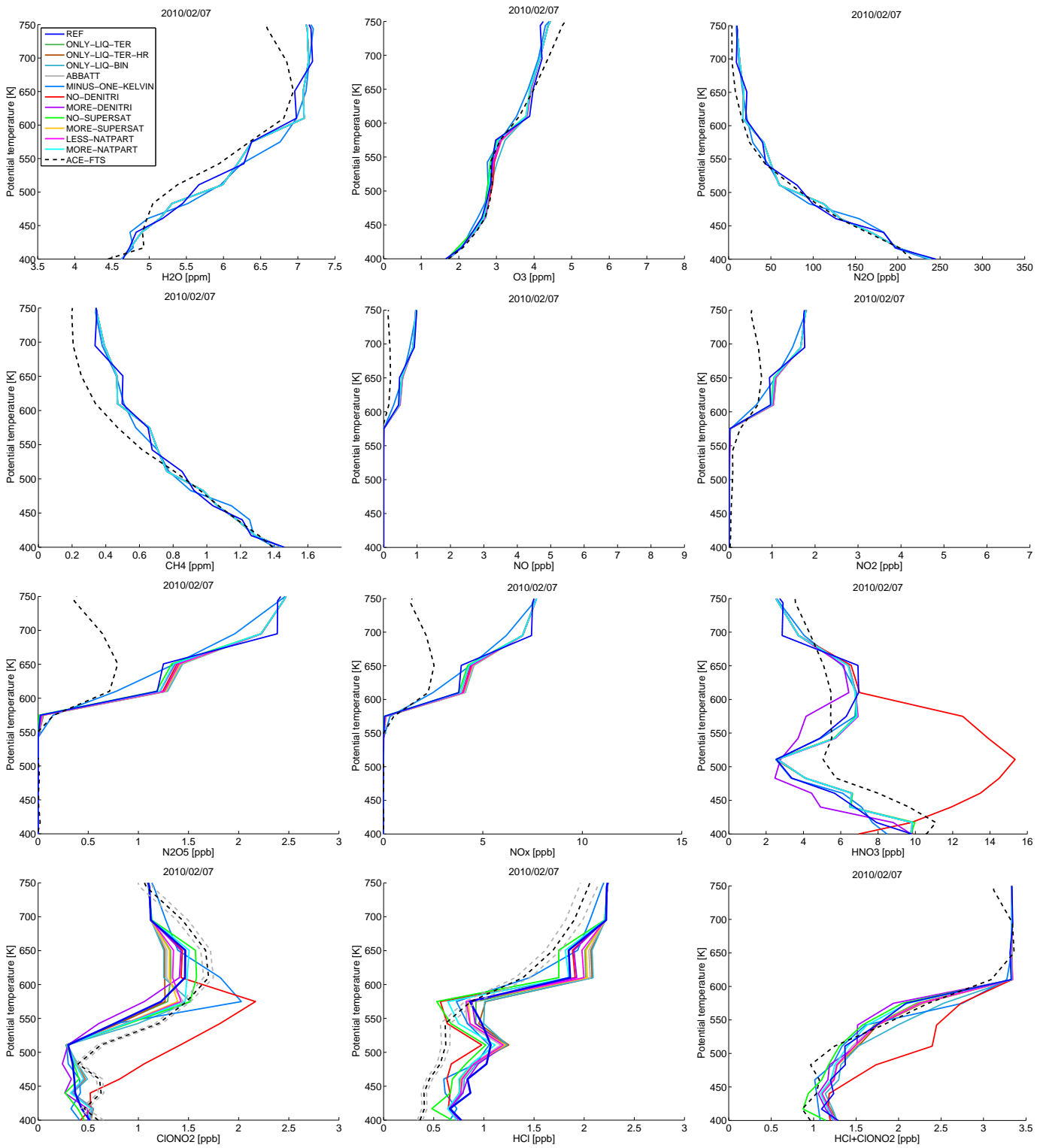
Figure 16: Example measurements of ACE-FTS on 7 February (67.4° N, 29.3° E) inside the vortex (black dashed lines). Profiles of H 2 O, O 3 , N 2 O, CH 4 , NO, NO 2 , N 2 O 5 , NO x = NO + NO 2 + 2N 2 O 5 , HNO 3 (gas phase), ClONO 2 , HCl and HCl + ClONO 2 . Colored lines show sensitivity runs (color code in the first figure).
