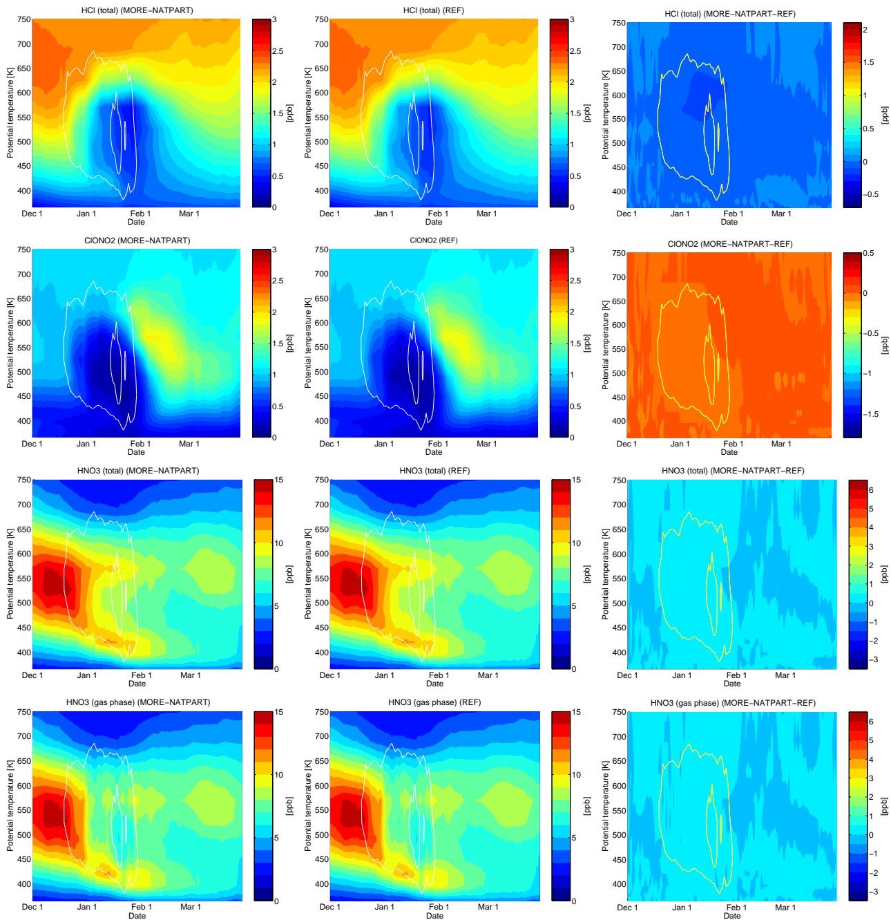
Figure 41: Vortex means as a function of model date and potential temperature inside the vortex boundary according to Nash. Left column: sensitivity run (MORE-NATPART), middle column: reference run, right column: difference (sensitivity minus reference run). From top to bottom: HCl, ClONO 2 , HNO 3 (total), HNO 3 (gas phase). White lines show the time periods where the formation of NAT clouds (outer line) and ice clouds (inner line) was possible inside the vortex.
