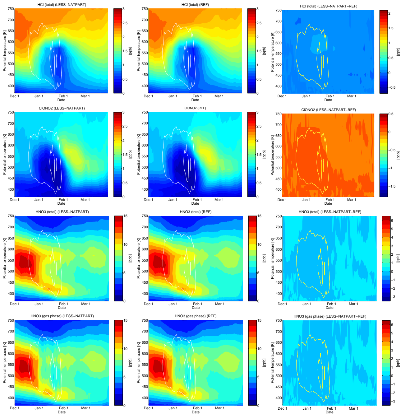
Figure 39: Vortex means as a function of model date and potential temperature inside the vortex boundary according to Nash. Left column: sensitivity run (LESS-NATPART), middle column: reference run, right column: difference (sensitivity minus reference run). From top to bottom: HCl, ClONO 2 , HNO 3 (total), HNO 3 (gas phase). White lines show the time periods where the formation of NAT clouds (outer line) and ice clouds (inner line) was possible inside the vortex.
