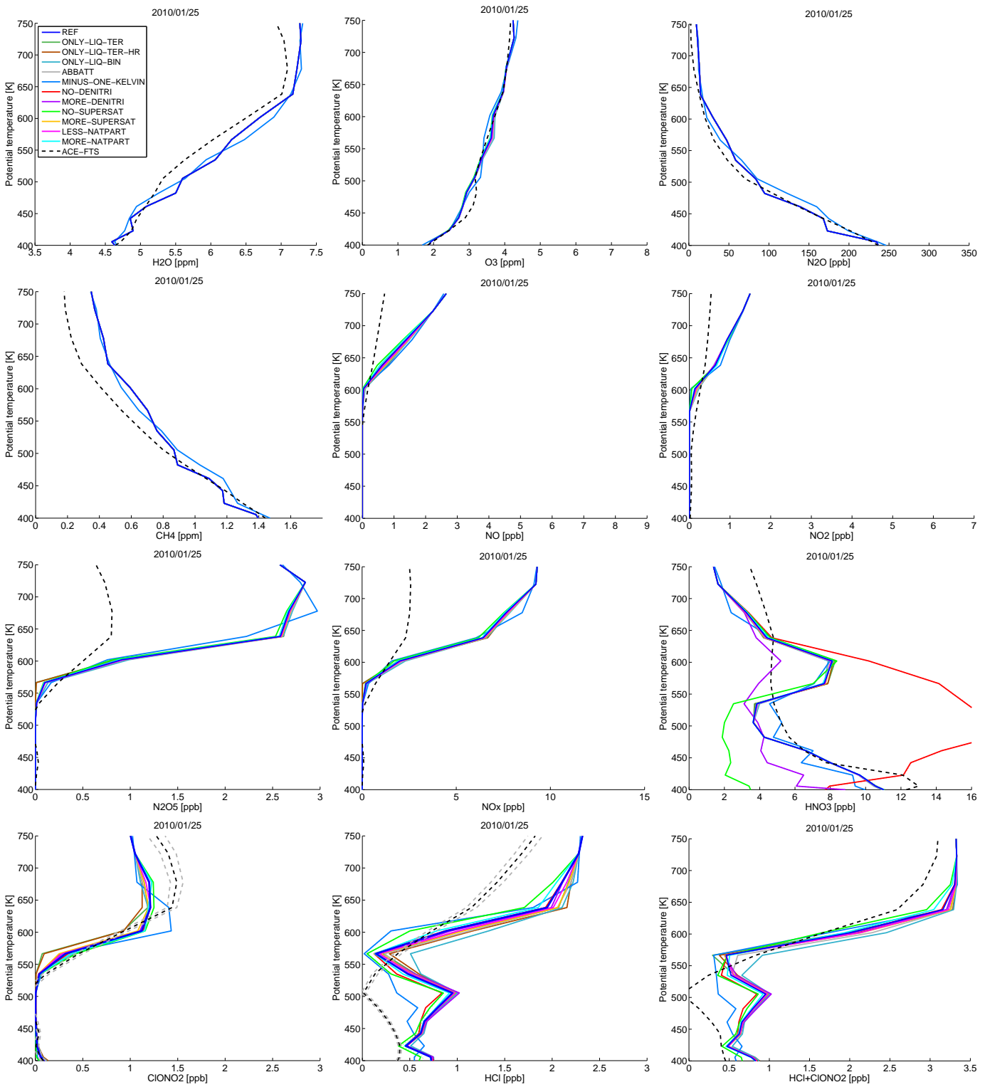
Figure 15: Example measurements of ACE-FTS on 25 January (65.2° N, 69.4° E) inside the vortex (black dashed lines). Profiles of H 2 O, O 3 , N 2 O, CH 4 , NO, NO 2 , N 2 O 5 , NO x = NO + NO 2 + 2N 2 O 5 , HNO 3 (gas phase), ClONO 2 , HCl and HCl + ClONO 2 . Colored lines show sensitivity runs (color code in the first figure).
