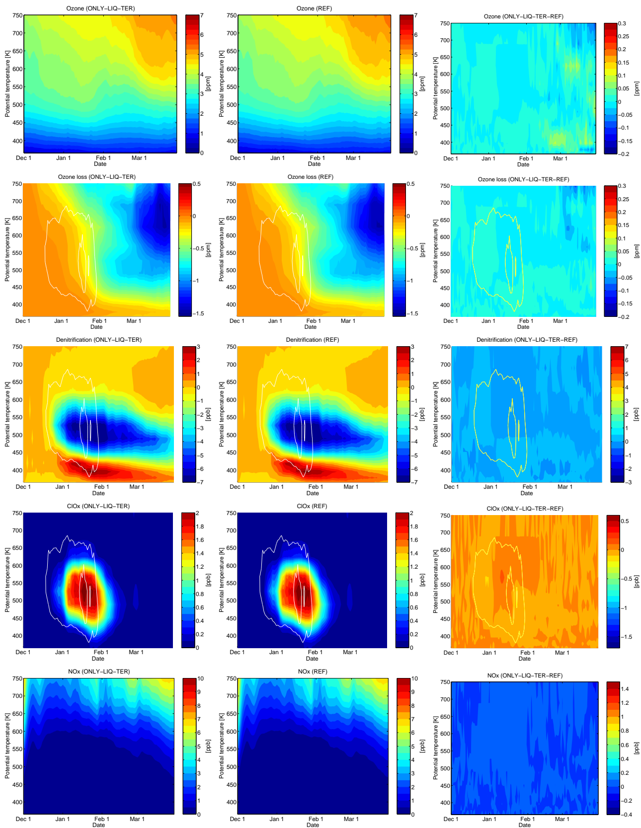
Figure 20: Vortex means as a function of model date and potential temperature inside the vortex boundary according to Nash. Left column: sensitivity run (ONLY-LIQ-TER), middle column: reference run, right column: difference (sensitivity minus reference run). From top to bottom: ozone, ozone loss (difference of ozone to passive tracer), denitrification (difference of \text{NO}_y to passive tracer), \text{ClO}_x and \text{NO}_x . White lines show the time periods where the formation of NAT clouds (outer line) and ice clouds (inner line) was possible inside the vortex.
