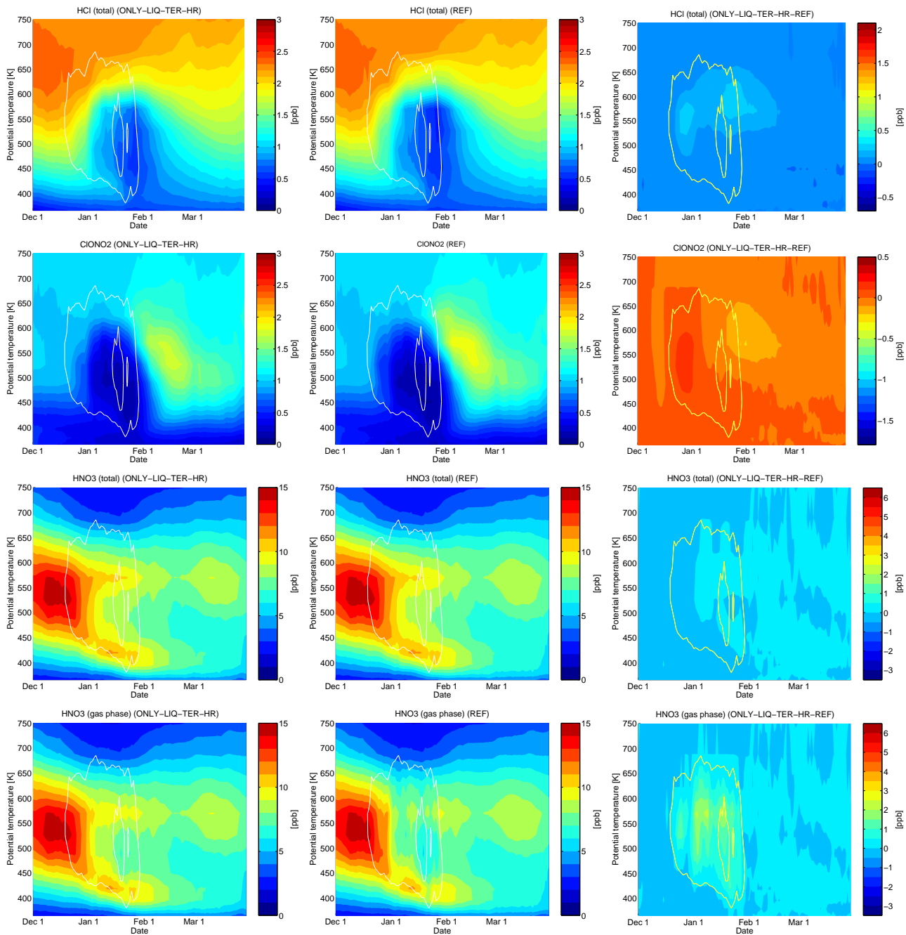
Figure 23: Vortex means as a function of model date and potential temperature inside the vortex boundary according to Nash. Left column: sensitivity run (ONLY-LIQ-TER-HR), middle column: reference run, right column: difference (sensitivity minus reference run). From top to bottom: HCl, ClONO 2 , HNO 3 (total), HNO 3 (gas phase). White lines show the time periods where the formation of NAT clouds (outer line) and ice clouds (inner line) was possible inside the vortex.
