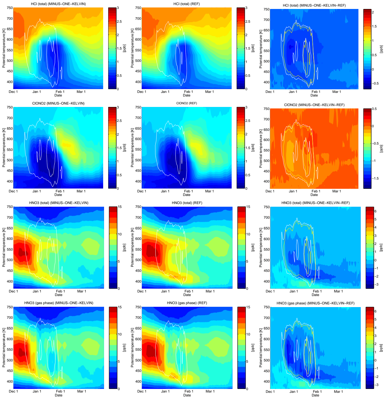
Figure 29: Vortex means as a function of model date and potential temperature inside the vortex boundary according to Nash. Left column: sensitivity run (MINUS-ONE-KELVIN), middle column: reference run, right column: difference (sensitivity minus reference run). From top to bottom: HCl, ClONO 2 , HNO 3 (total), HNO 3 (gas phase). White lines show the time periods where the formation of NAT clouds (outer line) and ice clouds (inner line) was possible inside the vortex.
