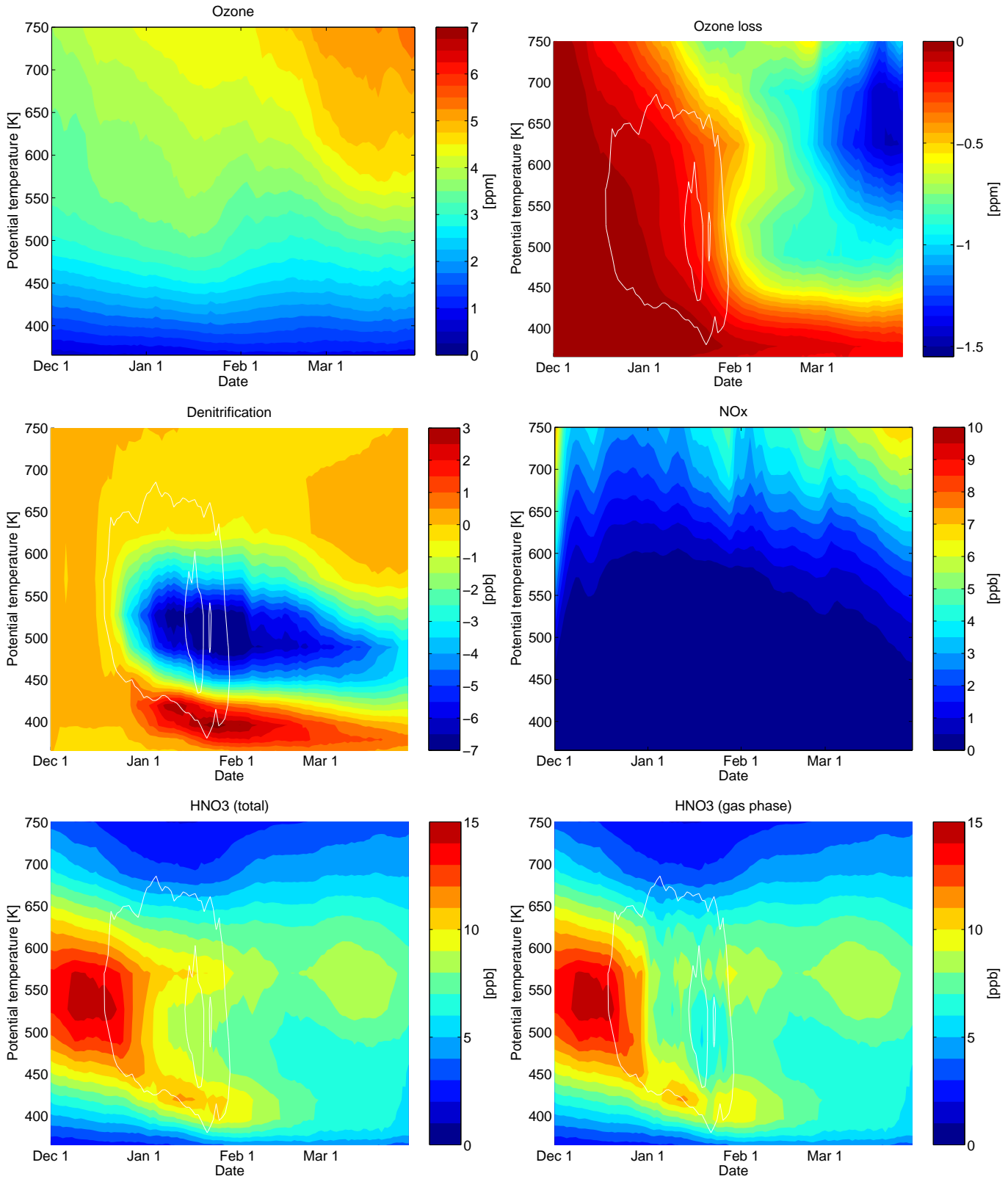
Figure 18: Vortex means as a function of model date and potential temperature inside the vortex boundary according to Nash. Ozone, ozone loss (difference of ozone to passive tracer), denitrification (difference of \text{NO}_y to passive tracer), \text{NO}_x , \text{HNO}_3 (total) and \text{HNO}_3 (gas phase). White lines show the time periods where the formation of NAT clouds (outer line) and ice clouds (inner line) was possible inside the vortex.
