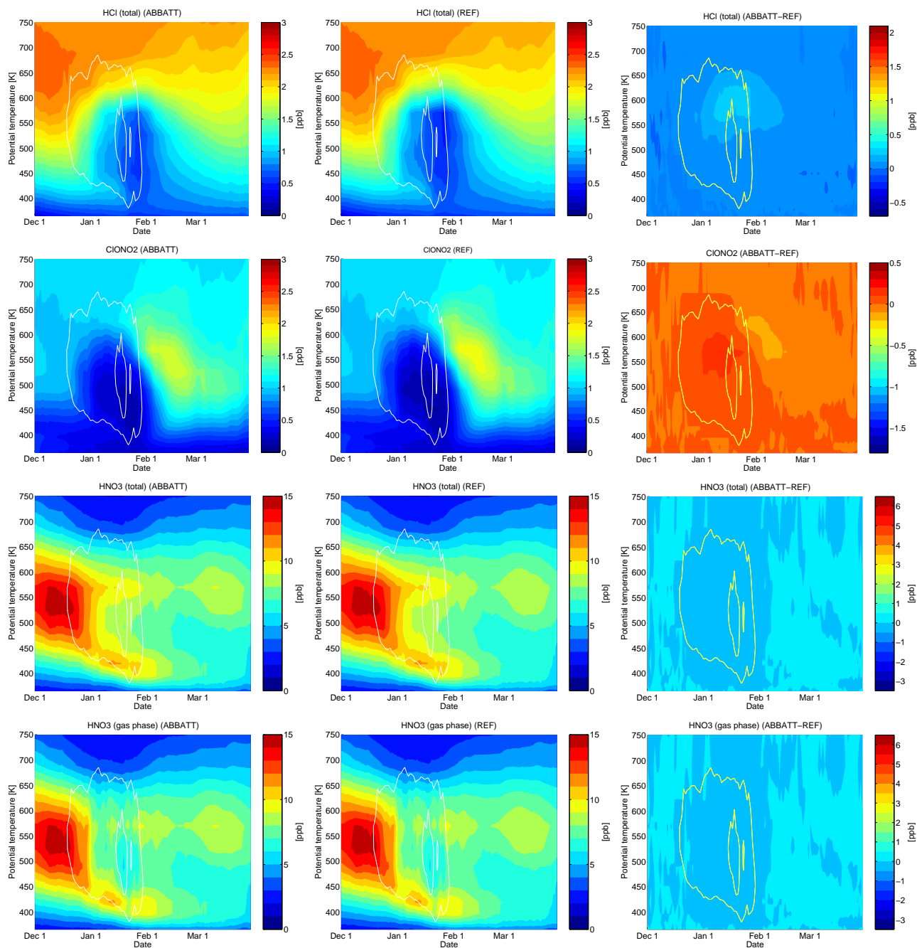
Figure 27: Vortex means as a function of model date and potential temperature inside the vortex boundary according to Nash. Left column: sensitivity run (ABBATT), middle column: reference run, right column: difference (sensitivity minus reference run). From top to bottom: HCl, ClONO 2 , HNO 3 (total), HNO 3 (gas phase). White lines show the time periods where the formation of NAT clouds (outer line) and ice clouds (inner line) was possible inside the vortex.
