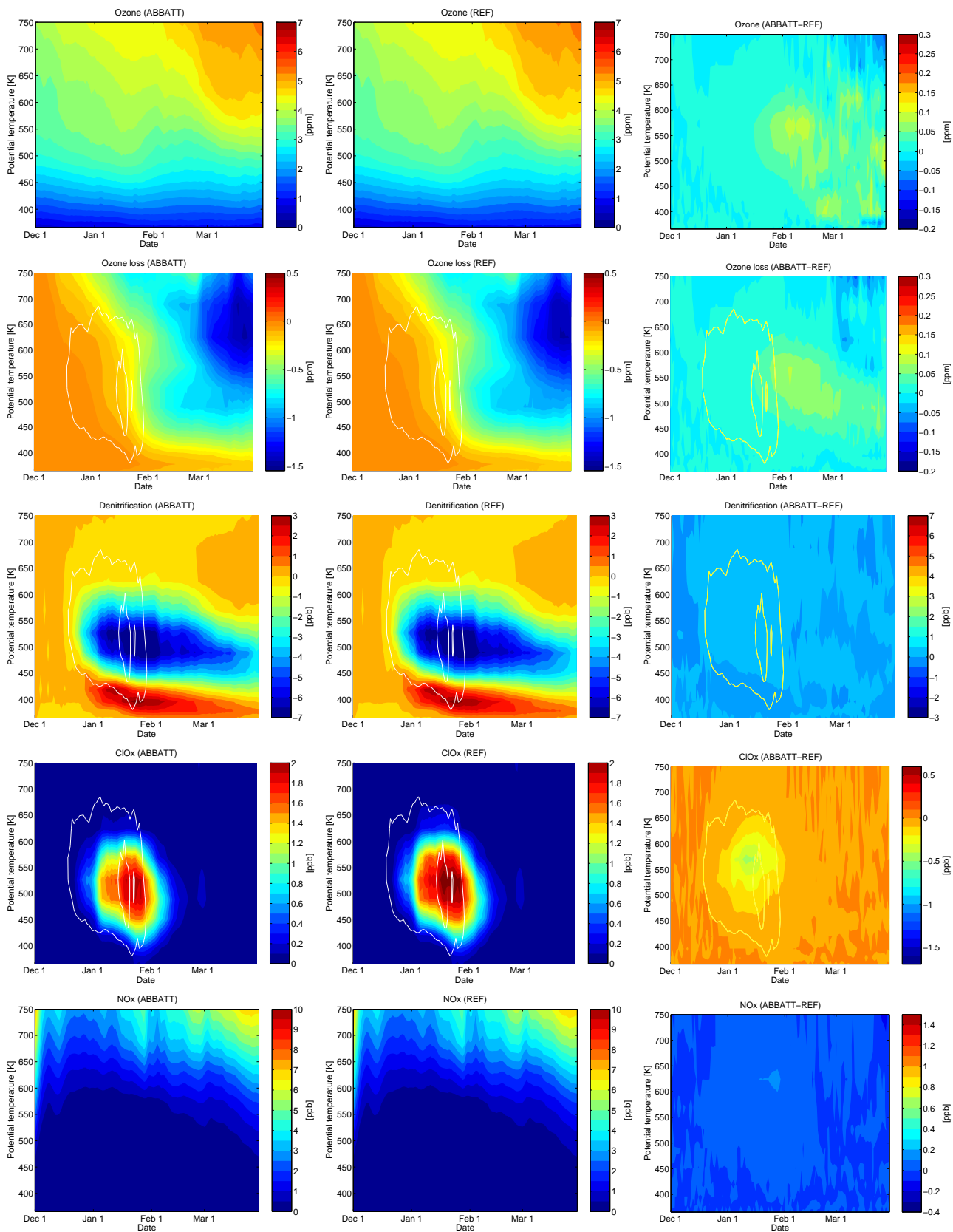
Figure 26: Vortex means as a function of model date and potential temperature inside the vortex boundary according to Nash. Left column: sensitivity run (ABBATT), middle column: reference run, right column: difference (sensitivity minus reference run). From top to bottom: ozone, ozone loss (difference of ozone to passive tracer), denitrification (difference of NO y to passive tracer), ClO x and NO x . White lines show the time periods where the formation of NAT clouds (outer line) and ice clouds (inner line) was possible inside the vortex.
