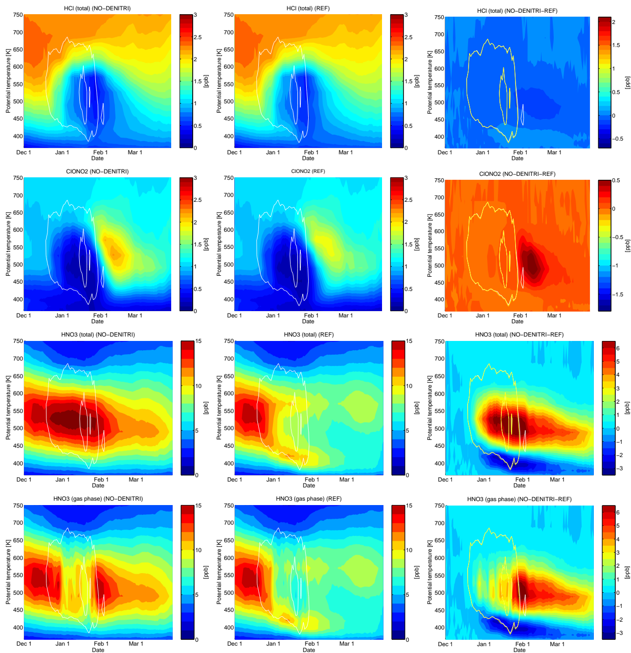
Figure 31: Vortex means as a function of model date and potential temperature inside the vortex boundary according to Nash. Left column: sensitivity run (NO-DENITRI), middle column: reference run, right column: difference (sensitivity minus reference run). From top to bottom: HCl, ClONO 2 , HNO 3 (total), HNO 3 (gas phase). White lines show the time periods where the formation of NAT clouds (outer line) and ice clouds (inner line) was possible inside the vortex.
