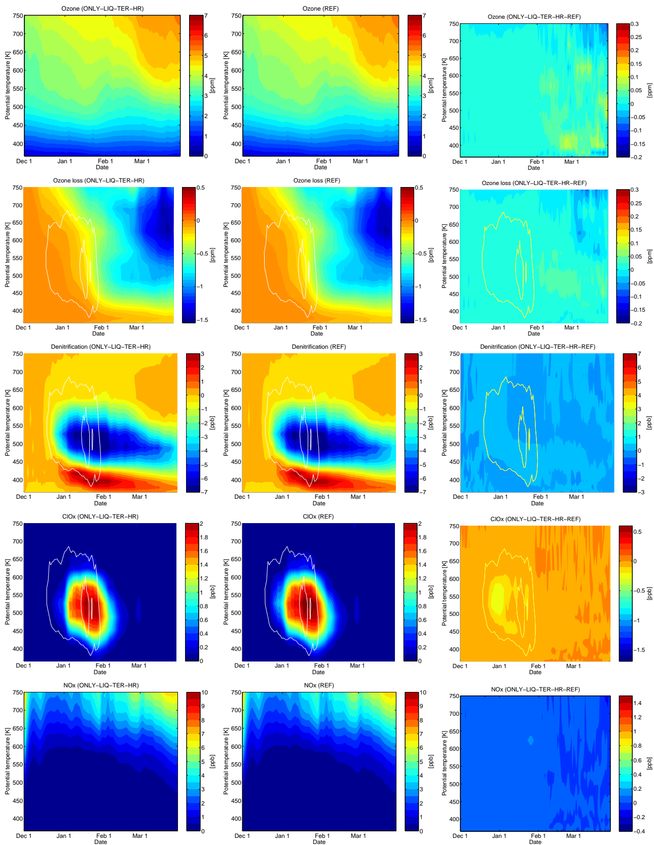
Figure 22: Vortex means as a function of model date and potential temperature inside the vortex boundary according to Nash. Left column: sensitivity run (ONLY-LIQ-TER-HR), middle column: reference run, right column: difference (sensitivity minus reference run). From top to bottom: ozone, ozone loss (difference of ozone to passive tracer), denitrification (difference of \text{NO}_y to passive tracer), \text{ClO}_x and \text{NO}_x . White lines show the time periods where the formation of NAT clouds (outer line) and ice clouds (inner line) was possible inside the vortex.
