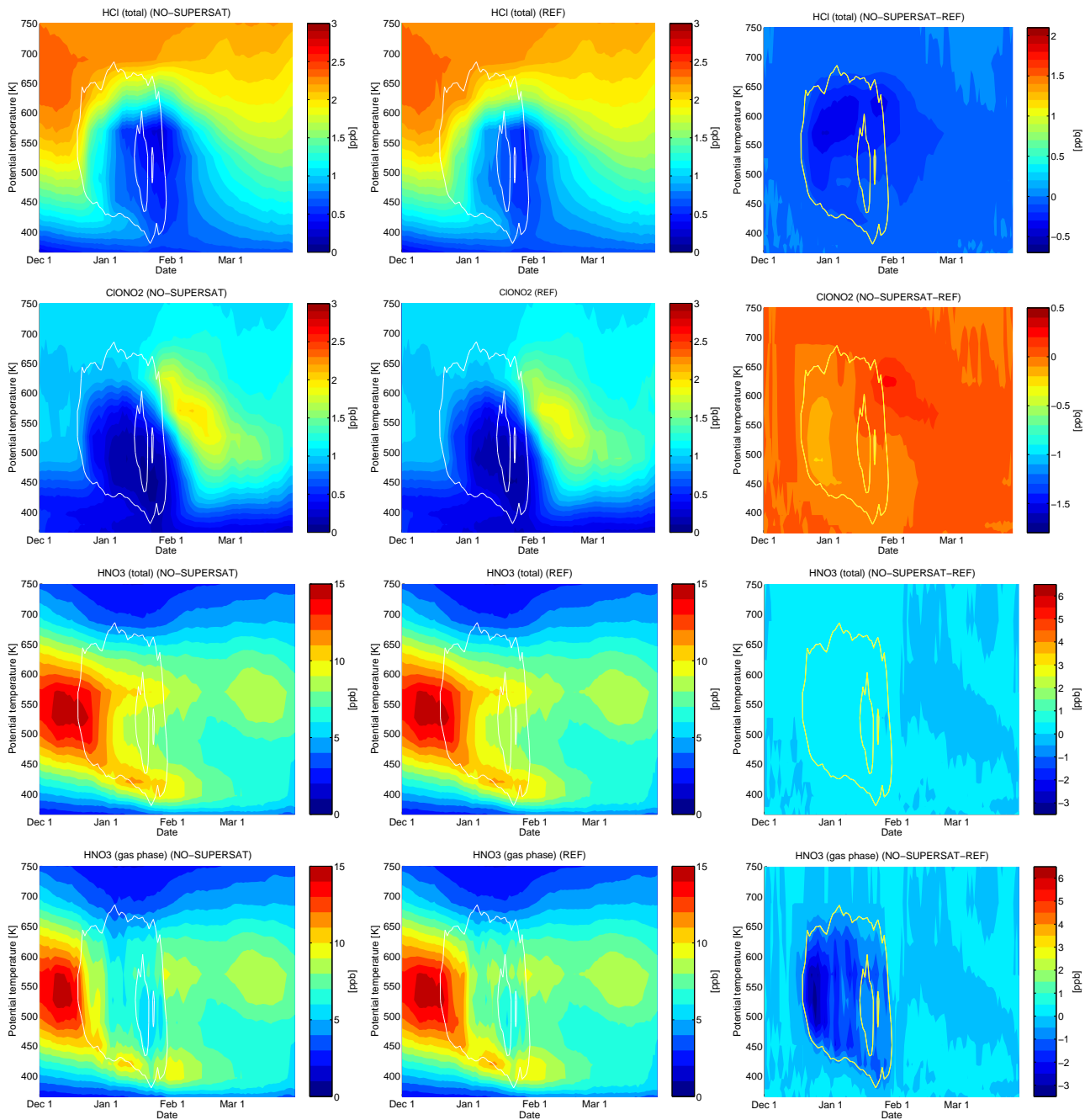
Figure 35: Vortex means as a function of model date and potential temperature inside the vortex boundary according to Nash. Left column: sensitivity run (NO-SUPERSAT), middle column: reference run, right column: difference (sensitivity minus reference run). From top to bottom: HCl, ClONO 2 , HNO 3 (total), HNO 3 (gas phase). White lines show the time periods where the formation of NAT clouds (outer line) and ice clouds (inner line) was possible inside the vortex.
