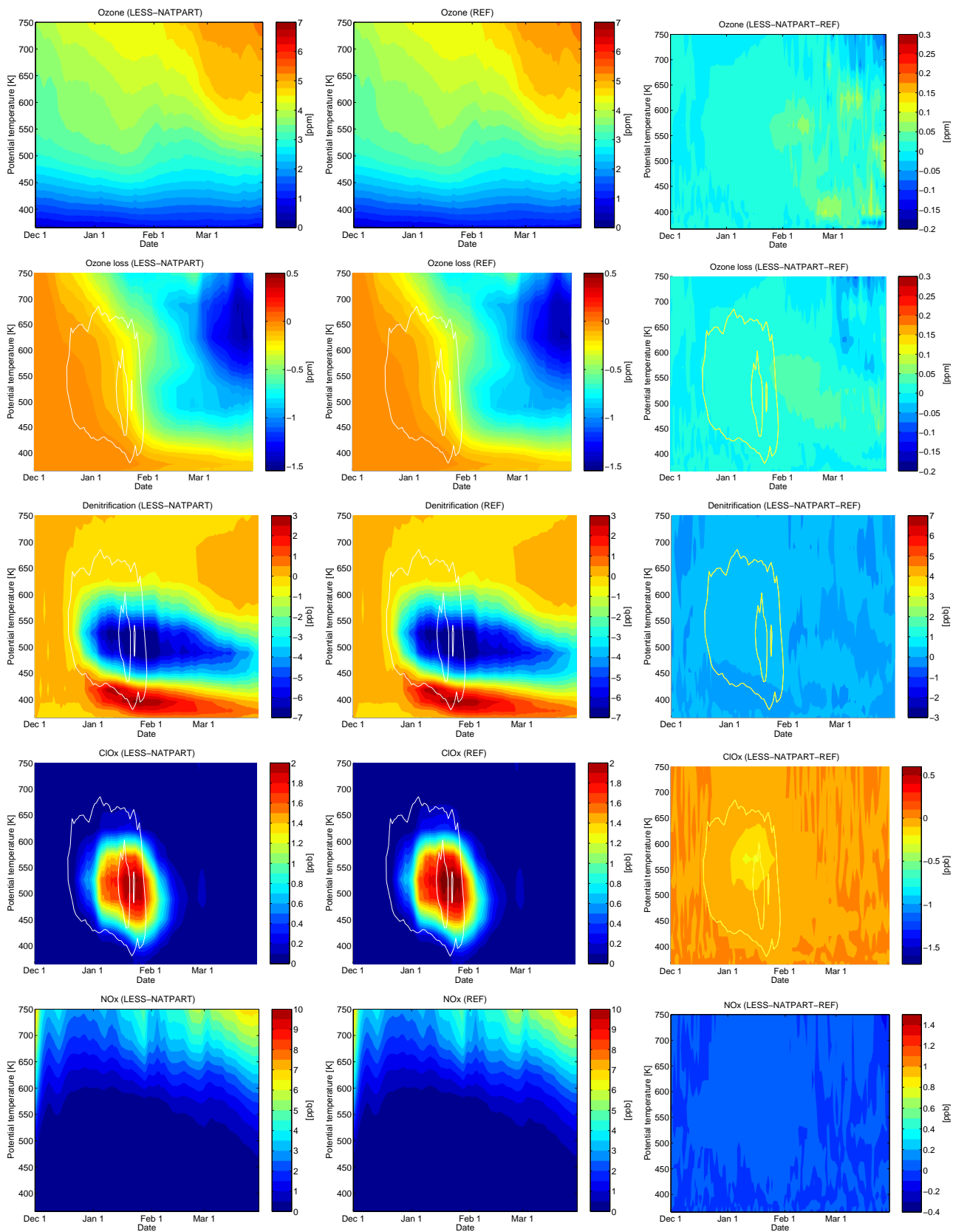
Figure 38: Vortex means as a function of model date and potential temperature inside the vortex boundary according to Nash. Left column: sensitivity run (LESS-NATPART), middle column: reference run, right column: difference (sensitivity minus reference run). From top to bottom: ozone, ozone loss (difference of ozone to passive tracer), denitrification (difference of NO y to passive tracer), ClO x and NO x . White lines show the time periods where the formation of NAT clouds (outer line) and ice clouds (inner line) was possible inside the vortex.
