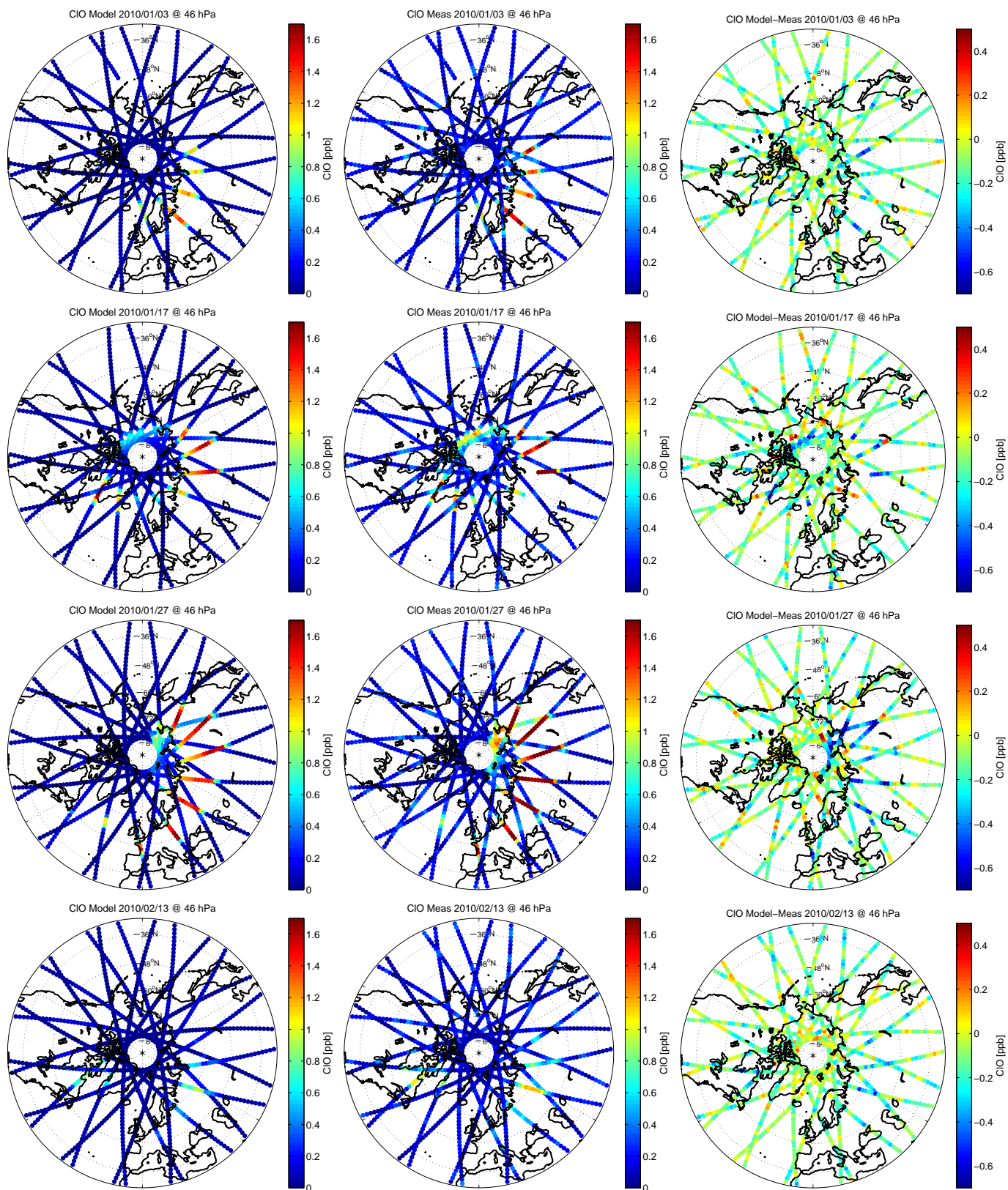
Figure 17: Modeled (left) and measured (middle) CIO mixing ratios at the MLS layer centered at 46 hPa along the satellite tracks. The rows show all measurements on 3 January, 17 January, 27 January and 13 February. The right column shows the differences. Backward trajectories starting at selected satellite measurements and ending at the time of the last model output before the measurement were calculated. Then, a chemical box model was initialized with the model data and the evolution of the species was calculated forward in time to obtain values to compare with the satellite measurements.
