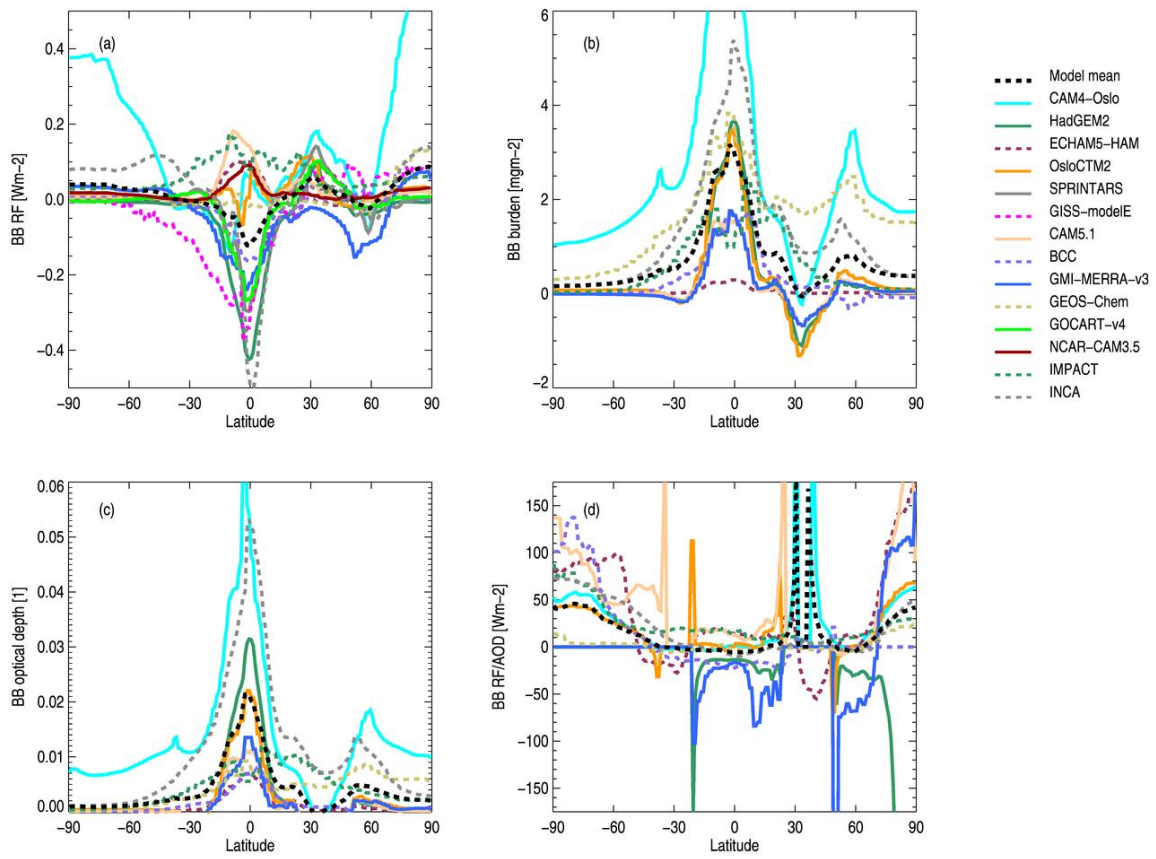
Figure S1: Zonal mean BB RF (a), burden (b), AOD at 550nm (c), NRF(A) (d)
