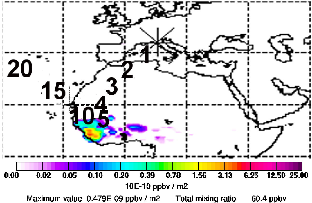
Figure S4. CO fire source contribution relative to ICO-OV observations on 29 th March 2009 (from 15 to 18 UTC). On the lower right is reported the CO fire mixing ratio simulated for the ICO-OV location. The numbers superimposed on the map are the days back in time for the retroplume centroid calculated by FLEXPART.
