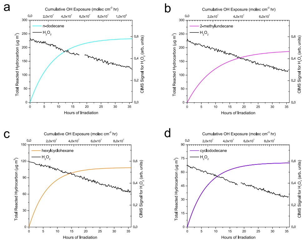
Figure S1: Total reacted hydrocarbon and H_2O_2 decay over experiment duration for (a) n-dodecane, (b) 2-methylundecane, (c) hexylcyclohexane, and (d) cyclododecane photooxidation.
