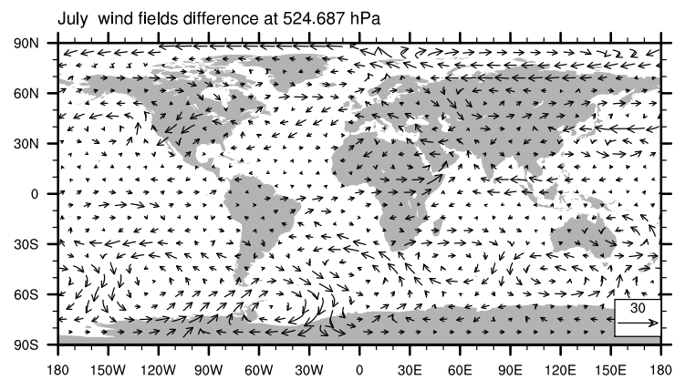
Figure S1 Wind fields differences (CAM5-AM3) in January and July at 957.486 hPa and 524.687 hPa.
