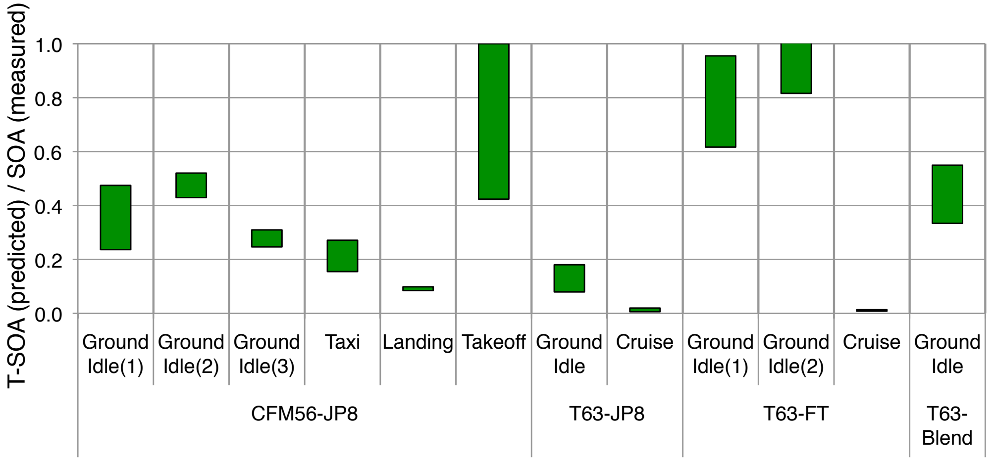
Figure S.1: Ratio of predicted T-SOA to measured SOA for all experiments.
