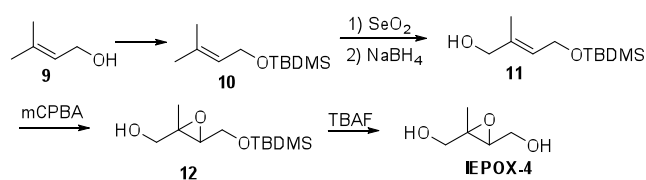
Fig. 4. Scheme for synthesis of IEPOX-4 . (Abbreviations: TBDMS, tert -butyldimethylsilyl; TBAF, tetrabutylammonium fluoride.)
