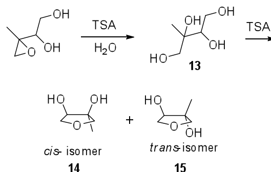
Fig. 5. Scheme for preparation of a mixture of 14 and 15 (method 1). (Abbreviation: TSA, toluenesulfonic acid.)
