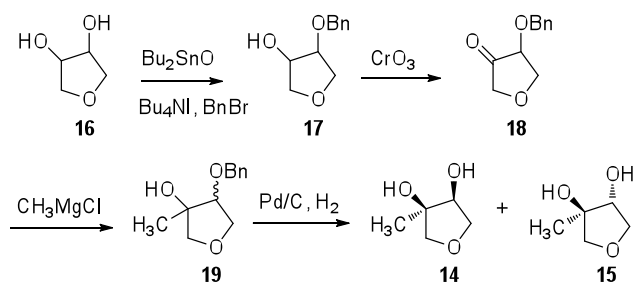
Fig. 6. Scheme for preparation of a mixture of 14 and 15 (method 2). (Abbreviation: Bu 2 SnO, dibutyltin oxide; Bu 4 NI, tetrabutylammonium iodide; BnBr, benzyl bromide.)
