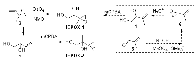
Fig. 2. Scheme for synthesis of IEPOX-1 and IEPOX-2 . The scheme within the box represents a multi-step procedure (Cole-Filipiak, 2010) for synthesis of IEPOX-1 in lower overall yield than in the present work. (Abbreviations: NMO, N -methylmorpholine oxide; m CPBA, m -chloroperbenzoic acid.)
