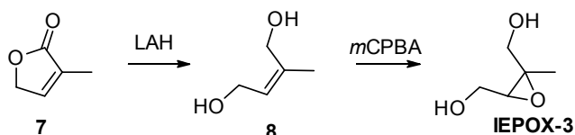
Fig. 3. Scheme for synthesis of IEPOX-3 . (Abbreviation: LAH, lithium aluminium hydride.)
