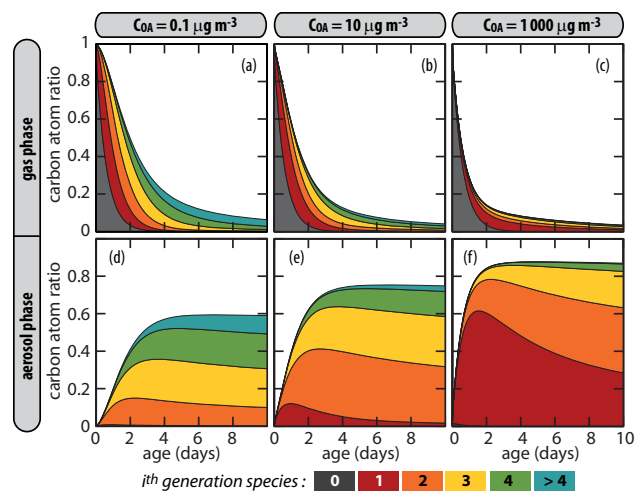
Fig. 3. Partitioning of organic carbon during hexadecane oxidation in the gas and aerosol phases as a function of C_{OA} . Colors identify the contribution of the species from a given generation to the total carbon budget.
