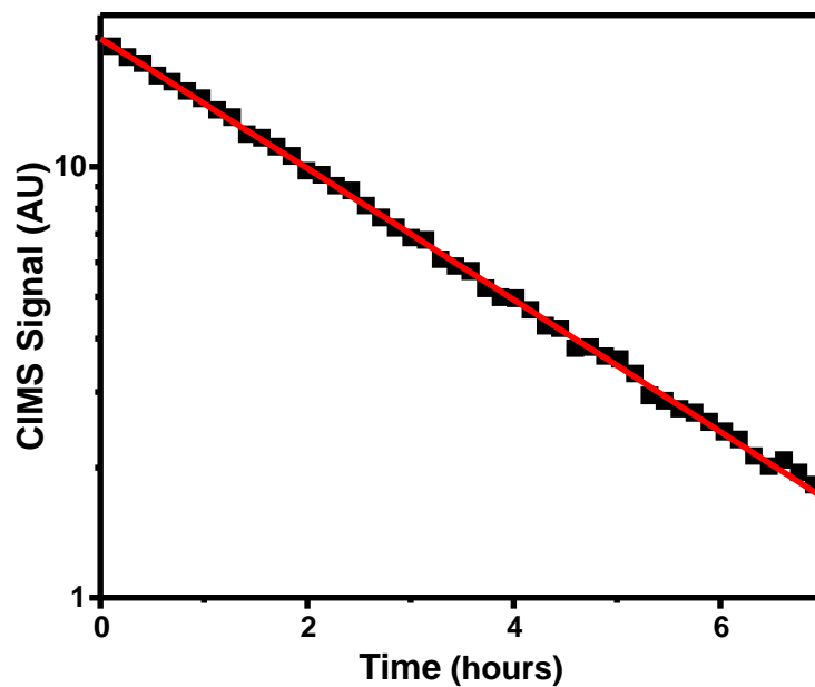
Figure S3 – Signal of pinonaldehyde from direct injection in the presence of 4 ppm H 2 O 2 photolyzed by black lights. The simulation (red line) incorporates both reaction with OH ( k_{\text{OH}} = 3.7 \times 10^{-11} \text{ cm}^3 \text{ molecules}^{-1} \text{ s}^{-1} ) and photolysis ( j = 7.26 \times 10^{-6} \text{ s}^{-1} ).
