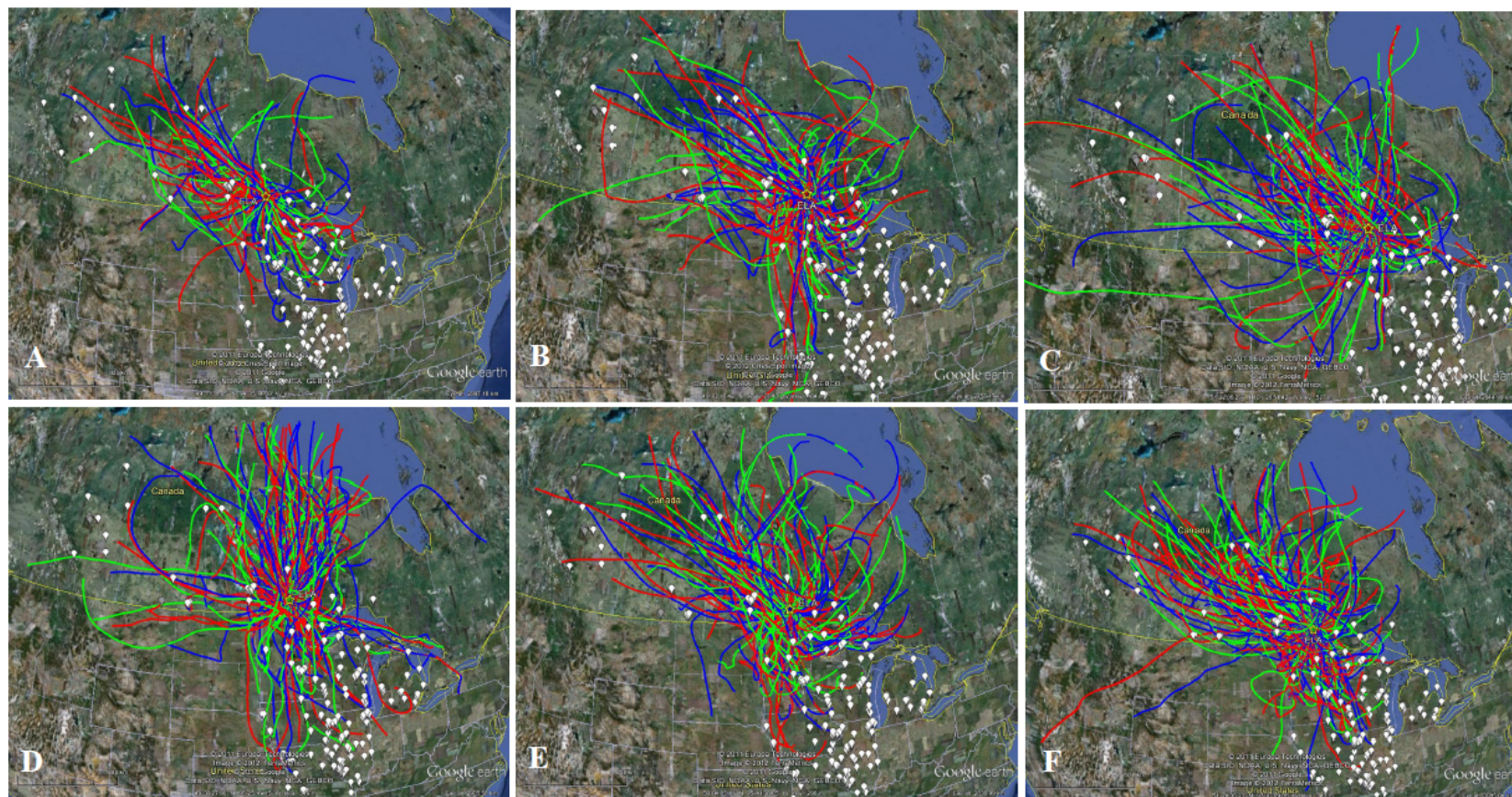
Fig. S1. Two-day HYSPLIT back trajectories for each season. (A) Summer05, (B) Fall05, (C) Winter06, (D) Spring06, (E) Summer06, and (F) Fall06. White placemarks represent Hg point sources. Winter months: December, January, February; Spring months: March, April, May; Summer months: June, July, August; Fall months: September, October, November.
