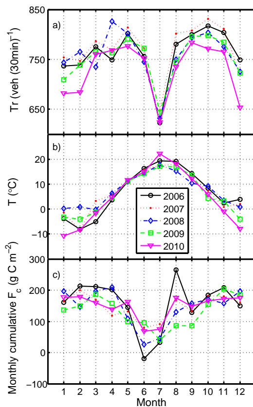
Fig. 3. Monthly mean (a) traffic rates and (b) air temperature, and (c) the monthly cumulative carbon flux separately for the studied years.
