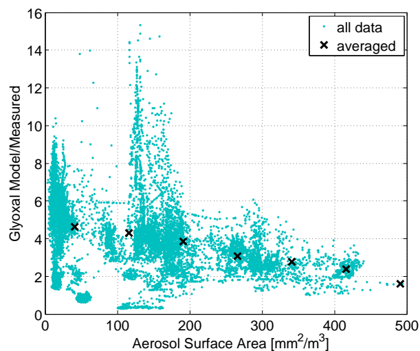
Fig. S2. Ratio of modelled to measured glyoxal as a function of aerosol surface area for model runs with no aerosol loss term for glyoxal. If aerosol loss corresponds to an important sink of glyoxal, model-measurement agreement should degrade at high aerosol surface areas. This is not the case, which shows that aerosol loss was not an important glyoxal sink during BEARPEX 2007. The analysis of daytime only values (not shown) produces the same result.
