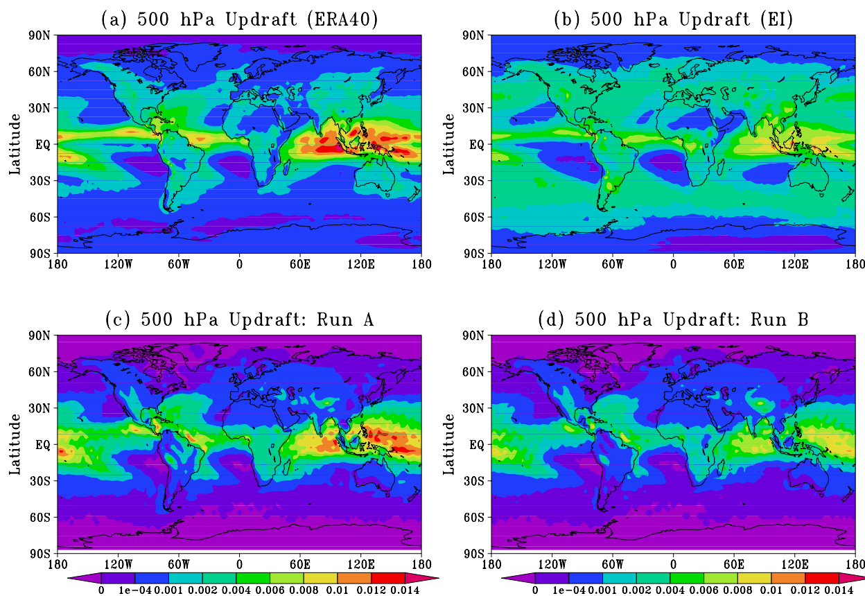
Fig. 1. Climatological convective updraft mass flux ( \text{kg m}^{-2} \text{s}^{-1} ) at 500 hPa averaged from (a) ERA-40 reanalyses (1989–2001), (b) ERA-Interim reanalyses (1989–2005), (c) run “A.E40” (1989–2005), and (d) run “B.EI” (1989–2005).
