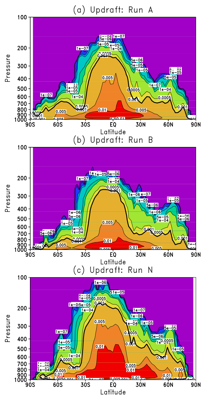
Fig. 5. Zonal mean convective updraft mass flux ( \text{kg m}^{-2} \text{s}^{-1} ) for runs (a) “A_E40”, (b) “B_EI”, and (c) “N_1991” averaged from 27 December 1990–11 January 1991. The bold contour indicates 0.001 \text{ kg m}^{-2} \text{ s}^{-1} .
