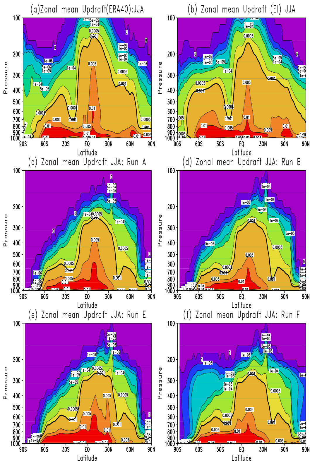
Fig. 3. Zonal mean convective updraft mass flux ( \text{kg m}^{-2} \text{s}^{-1} ) averaged for JJA from (a) ERA-40 reanalyses (1989–2001), (b) ERA-Interim reanalyses (1989–2005), (c) run “A_E40” (1989–2005), (d) run “B_EI” (1989–2005), (e) run “E_EInewevap” (1989–2005), and (f) run “F_EInewconv” (1989–2005). The bold contour indicates 0.001 \text{ kg m}^{-2} \text{ s}^{-1} .
