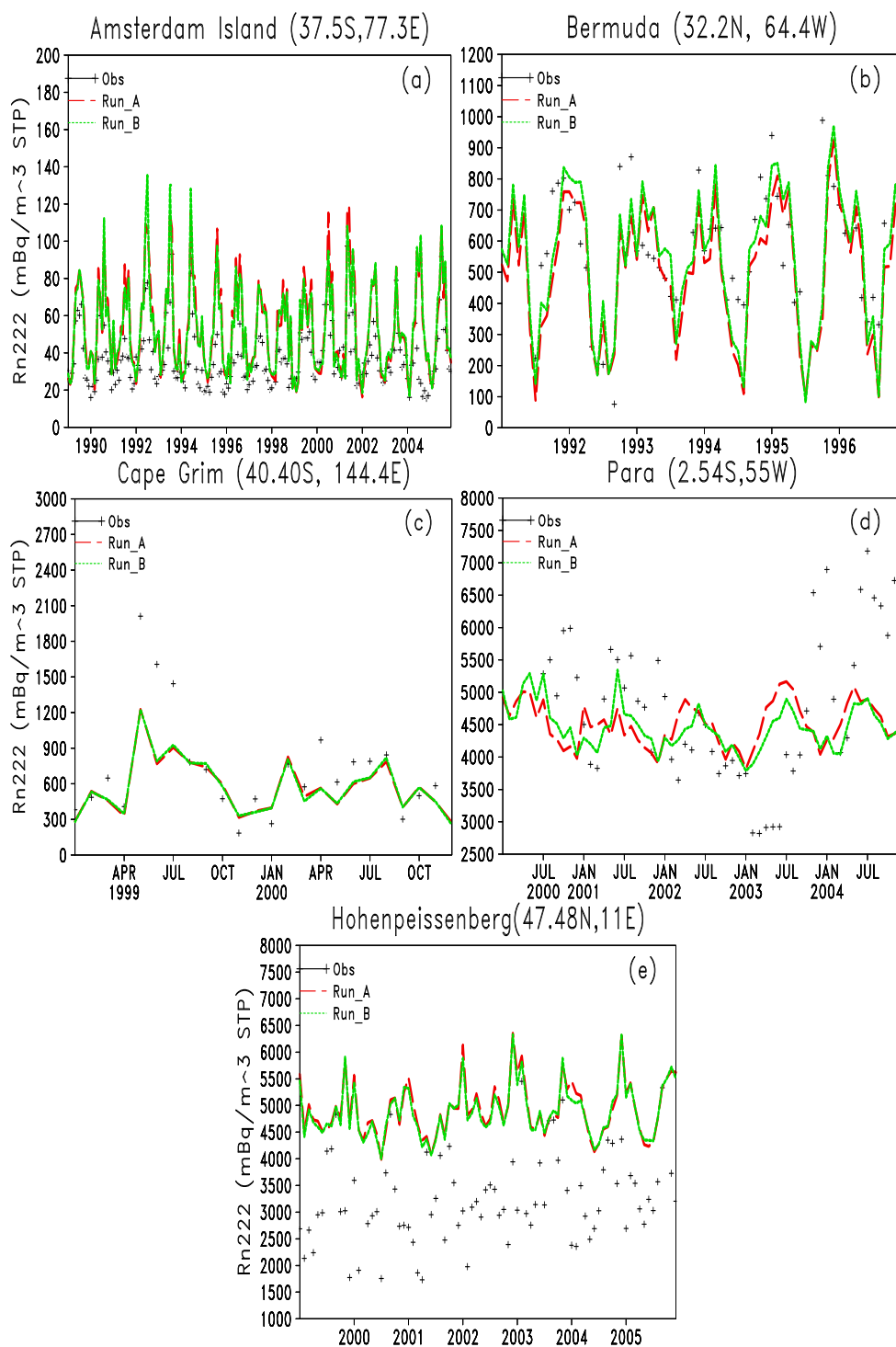
Fig. 12. Comparison of observed surface radon concentrations ( \text{mBq/m}^3 STP) with model runs “A_E40” and “B_EI” at (a) Amsterdam Island ( 37.5^\circ S, 77.3^\circ E), (b) Bermuda ( 32.2^\circ N, 295.6^\circ E). (c) Cape Grim ( 40.4^\circ S, 144.4^\circ E), (d) Par , Brazil ( 2.5^\circ S, 305^\circ E), and (e) Hohenpeissenberg ( 47.5^\circ N, 11^\circ E). Note different x-axis and y-axis scales.
