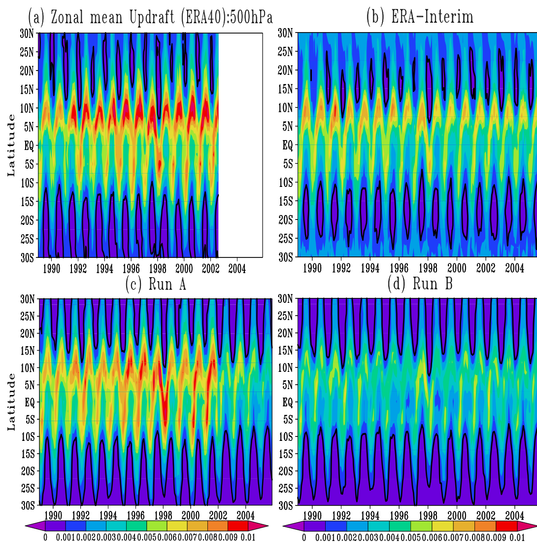
Fig. 2. Time series of zonal mean monthly mean updraft convective mass flux ( \text{kg m}^{-2} \text{s}^{-1} ) at 500 hPa from (a) ERA-40 reanalyses, (b) ERA-Interim reanalyses, (c) Run “A_E40” (forced by operational winds from 2002 onwards), and (d) Run “B_EI”. The bold contour indicates 0.001 \text{ kg m}^{-2} \text{ s}^{-1} .
