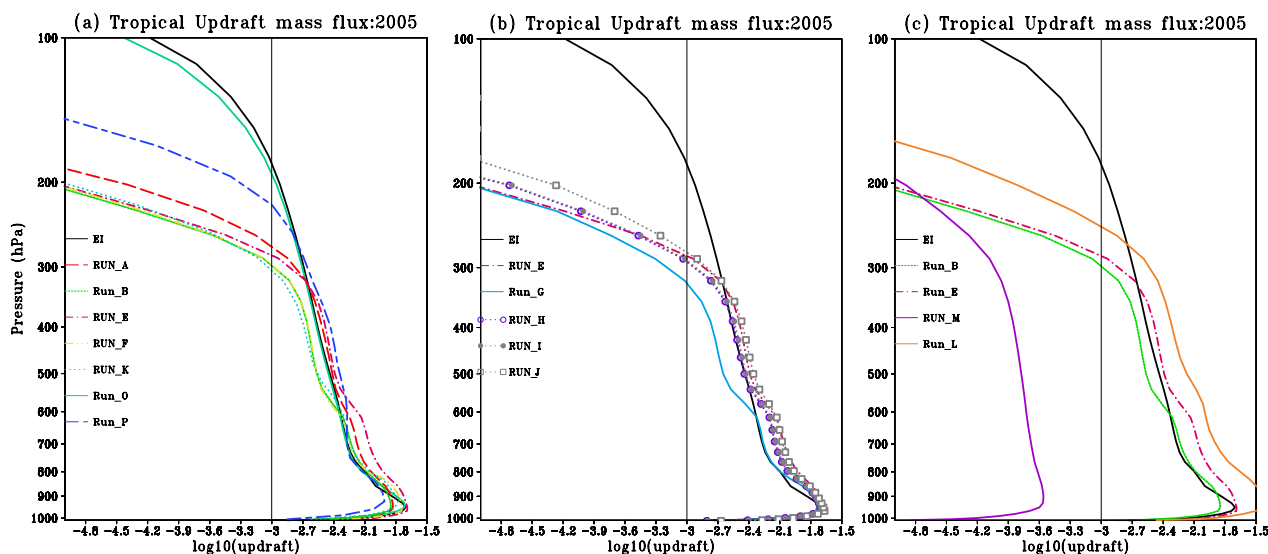
Fig. 7. Zonal mean annual mean tropical ( 25^{\circ} S– 25^{\circ} N) updraft convective mass flux ( \text{kg m}^{-2} \text{s}^{-1} ) for 2005 from ERA-Interim reanalyses and (a) runs “A_E40”, “B_EI”, “E_EInewevap”, “F_EInewconv”, “K_L31”, “N_1991” (December 1990 to January 1991), “O_EIar”, “P_det”, (b) runs “E_EInewevap”, “G_5.6”, “H_1.1”, “I_1.4”, “J_T106”, and (c) runs “B_EI”, “E_EInewevap”, “L_2EVAP”, “M_0EVAP”.
