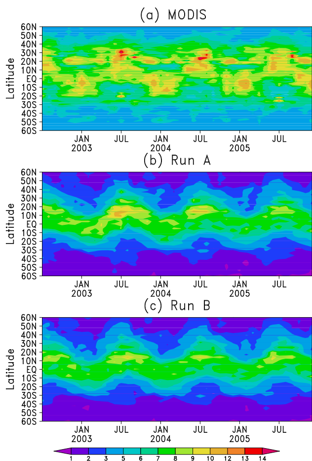
Fig. 8. Time series of monthly mean cloud top height (km) from (a) MODIS (b) run “A_E40”, and (c) run “B_EI”.
