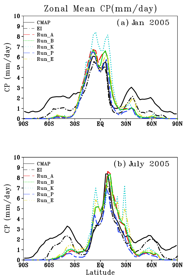
Fig. 11. Zonal mean convective precipitation (mm/day) from CMAP data, ERA-Interim reanalyses and model runs “A_E40”, “B_EI”, “K_L31”, “P_det” and “E_EInewevap” for (a) January 2005, and (b) July 2005.
