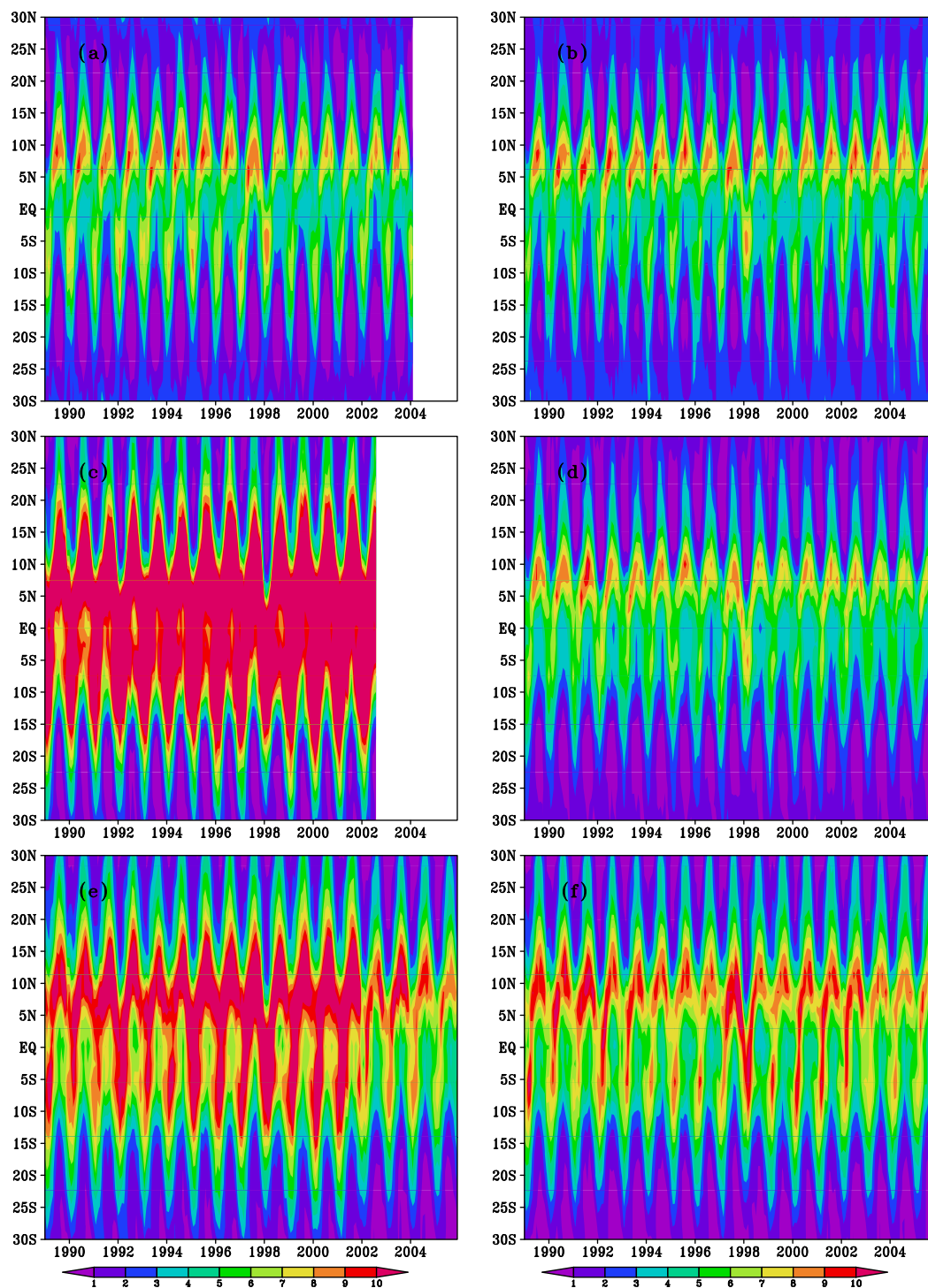
Fig. 10. Zonal mean convective precipitation (mm/day) from (a) GPI data, (b) CMAP data, (c) ERA-40 reanalyses, (d) ERA-Interim reanalyses, (e) run “A_E40”, and (f) run “B_EI”.
