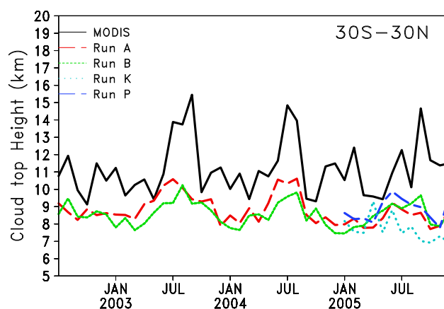
Fig. 9. Time series of monthly mean maximum daily cloud top height (km) for 2002–2005 averaged between 30° S–30° N from MODIS and model runs “A_E40”, “B_EI”, “K_L31” and “P_det”.
