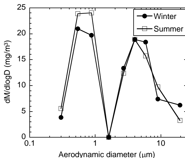
Fig. 1. Size distribution of the aerosol mass during winter (21 January to 12 February 2002) and summer (28 July to 13 August 2002) at Tsukuba, Japan.
