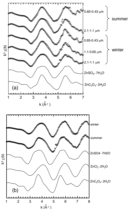
Fig. 6. Zinc K-edge EXAFS spectra (open circles = sample, lines = fitting) of finer particles during winter and summer at Tsukuba with standard materials used for fitting: (a) 2.1–1.1, 1.1–0.65 and 0.65–0.43 \mu\text{m} in winter, and 2.1–1.1 and 0.65–0.43 \mu\text{m} in summer, and (b) 3.3–2.1 \mu\text{m} in winter and summer.
