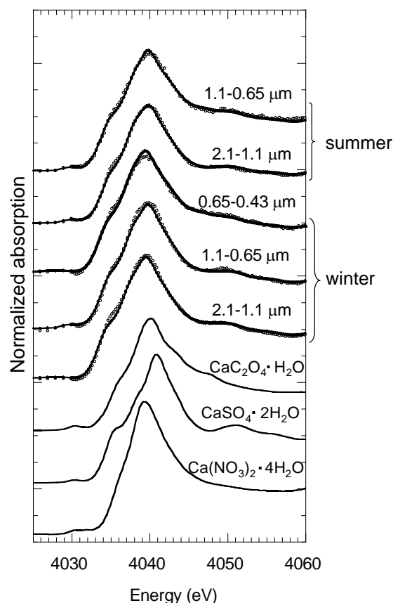
Fig. 4. Calcium K-edge XANES spectra (open circles = samples, lines = fitting) of finer particles during winter and summer at Tsukuba with those of the standard materials used for fitting.
