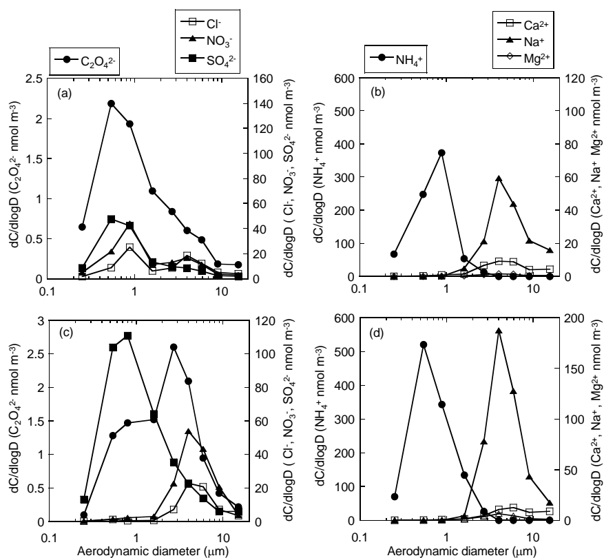
Fig. 2. Size distribution of WSCs in aerosols at Tsukuba: (a) anions and (b) cations in winter; (c) anions and (d) cations in summer.
