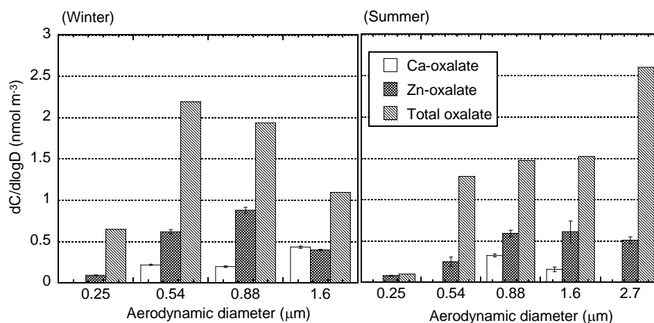
Fig. 7. Atmospheric concentrations of Ca oxalate, Zn oxalate, and total oxalate during winter and summer.
