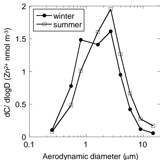
Fig. 3. Size distribution of Zn in aerosols during winter and summer at Tsukuba.
