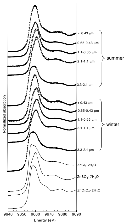
Fig. 5. Zinc K-edge XANES spectra (open circles = samples, lines = fitting) of finer particles during winter and summer at Tsukuba with those of the standard materials used for fitting.
