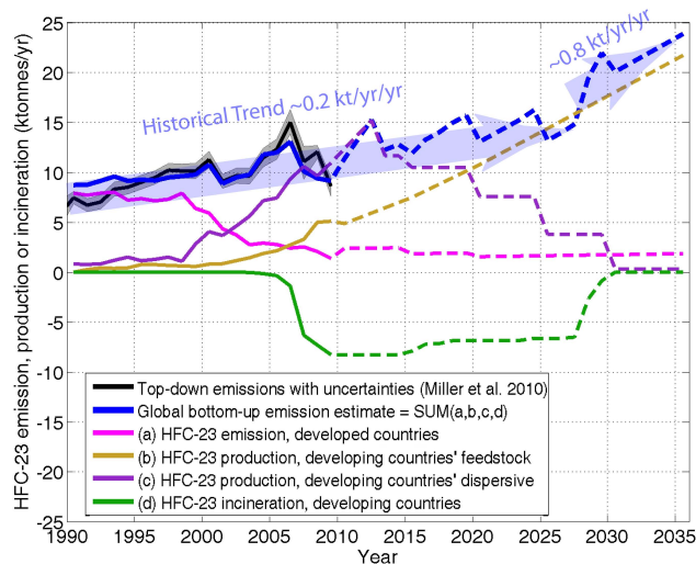
Fig. 1. Bottom-up HFC-23 emissions for developed countries (solid line a) (UNFCCC, 2010), and HFC-23 production and incineration for developing countries (solid lines b–d) (Miller et al., 2010), shown along with the bottom-up global HFC-23 emissions, which are the annual sums of each of these components. The bottom-up emissions, production and incineration are projected (dotted lines) to 2035 based on the “Reference Case” (RC) assumptions. The RC scenario suggests that the historical trend in emission growth of \sim 0.2 ktonnes \text{yr}^{-2} continues over much of the coming two decades. CDM project accreditation is scheduled to end by 2030, after which global emission growth quadruples to \sim 0.8 ktonnes \text{yr}^{-2} and is controlled indefinitely by the unrestricted production of HCFC-22 for feedstock use. Note that this increase occurs despite the complete phase out of HCFC-22 for dispersive uses by 2030. The top-down global emission estimates of Miller et al. (2010) (solid black line with uncertainties in gray) are shown as emission verification of the global bottom-up estimate.
