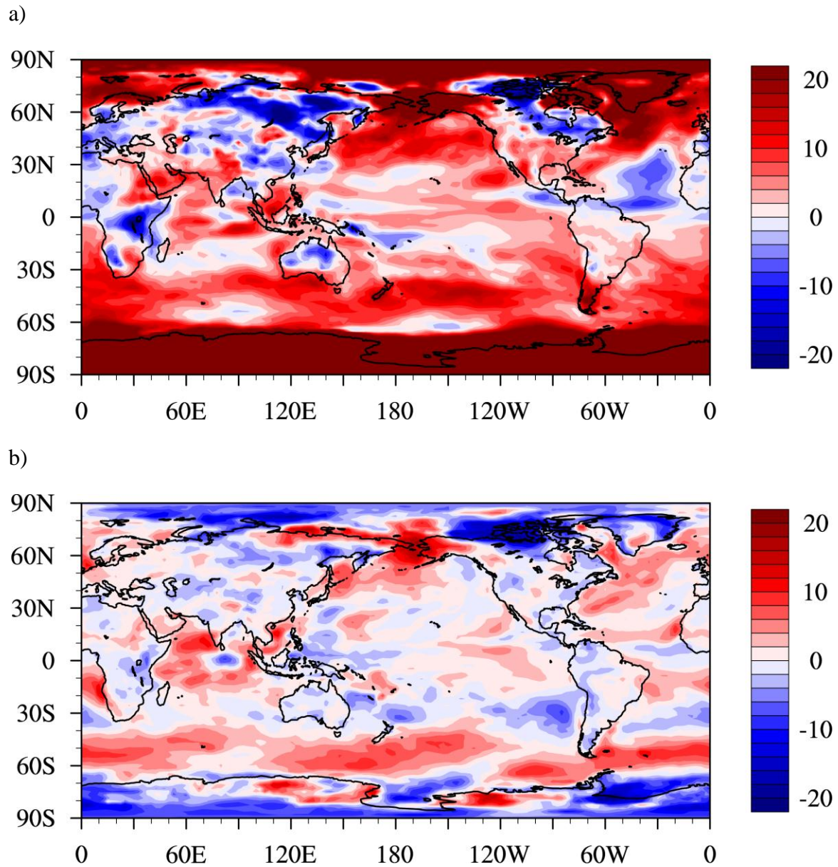
Fig. S2. Annual average percentage change in surface CCN concentration at a) 0.01% and b) 1% supersaturation between the Default and G11 simulations.
