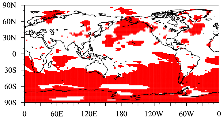
Fig. S1. The results of the paired t-test ( P < 0.05 ) between marine-source submicron OM concentration and CCN number changes for a) G11 and b) V10 simulations.
