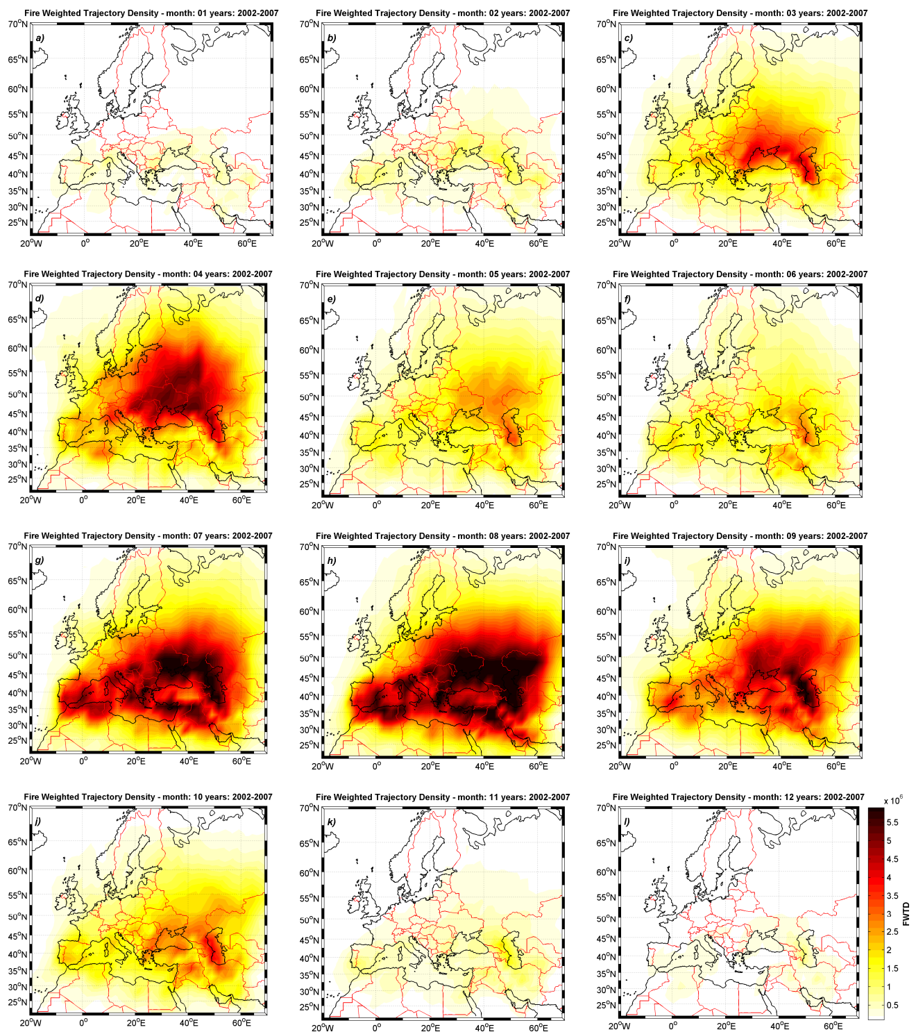
Figure S1: FWTD fields obtained for the 12 months of the year (panels a to l) as average over the 2002-2007 period.
