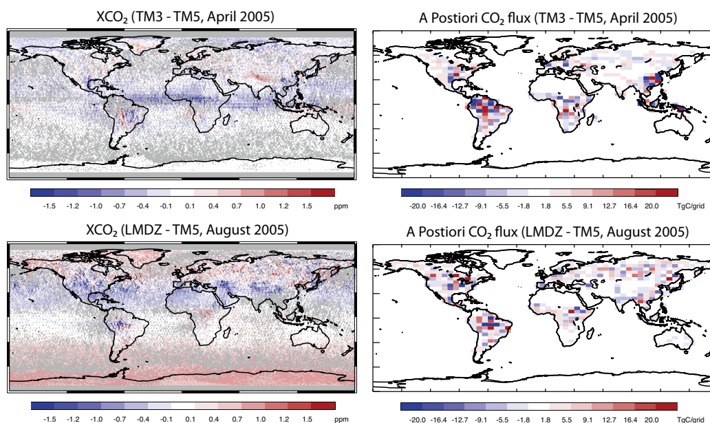
Fig. 6. Examples of the inversion-derived mapping of concentration differences to flux differences. Top panels: TM5 inversion using TM3-derived x\text{CO}_2 samples for April. Bottom panels: TM5 inversion using LMDZ-derived x\text{CO}_2 samples for August.
