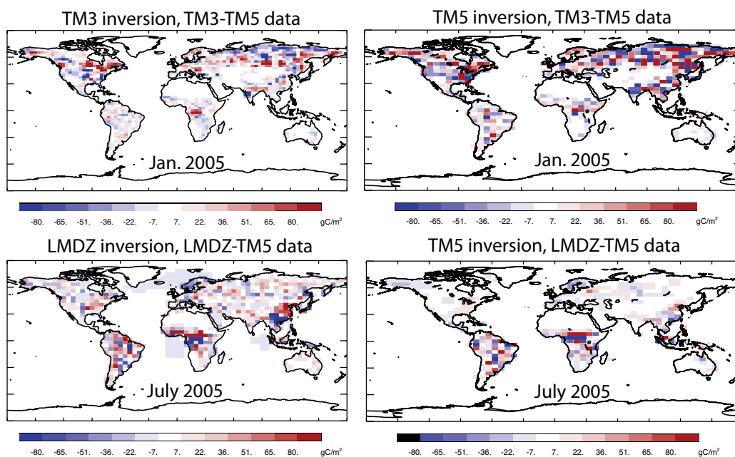
Fig. 7. Examples fluxes derived from different inversion using the same samples. Top panels: TM5 and TM3 inversion using the difference between TM5 and TM3 derived A-SCOPE samples for January. Bottom panels: TM5 and LMDZ inversion using the difference between TM5 and LMDZ derived A-SCOPE samples for July.
