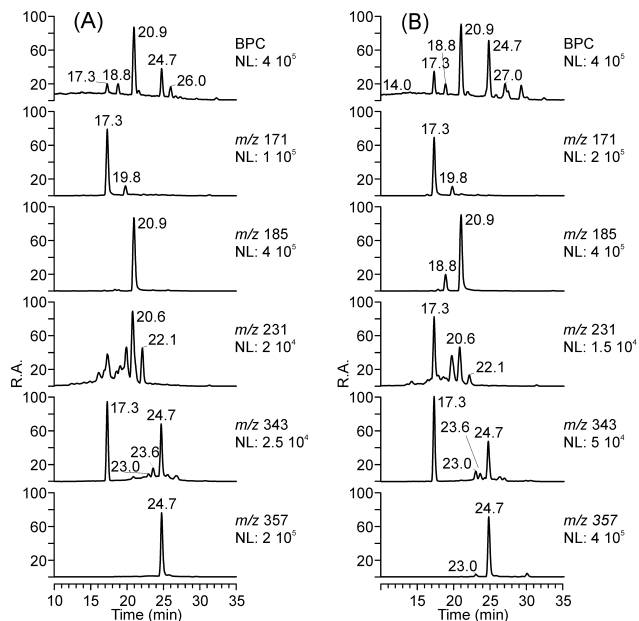
Fig. 1. LC/MS chromatographic data [base peak chromatograms (BPCs) and extracted ion chromatograms (EICs)] for (A) \alpha -pinene and (B) \beta -pinene ozonolysis SOA. Abbreviation: NL, normalization level.
