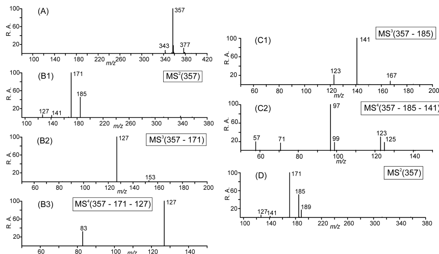
Fig. 5. (–)ESI-MS data for the major MW 358 compound [RT 24.7 min; Fig. 1(B)] present in \beta -pinene ozonolysis SOA, assigned to a covalent dimer of the ester type: (A) first-order mass spectrum; (B1) m/z 357 MS^2 spectrum; (B2) and (B3) m/z 357 \rightarrow m/z 171 MS^n ( n = 3, 4 ) spectra; and, (C1) and (C2) m/z 357 \rightarrow m/z 185 MS^n ( n = 3, 4 ) spectra. (D) m/z 357 MS^2 spectrum for the minor MW 358 compound at RT 23.0 min (Fig. 1b).
