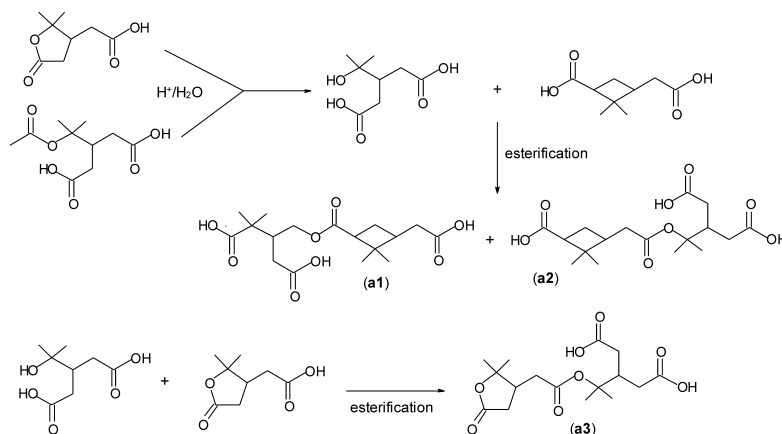
Scheme 2. Proposed formation mechanism for the MW 358 and 344 compounds related to terpenylic acid and diaterpenylic acid acetate.
