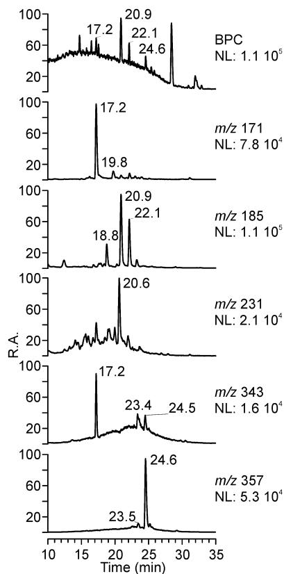
Fig. 2. LC/MS chromatographic data (BPC and EICs) for fine ambient aerosol ( PM_{2.5} ) from K-pusztá, Hungary, collected during the night of 19 June 2006 of the warm period of the 2006 summer field campaign. The peak at RT 22.1 min (not discussed in the main text) on the m/z 185 EIC is tentatively assigned to cis -caronic acid, a positional isomer of cis -pinic acid, based on comparison of its chromatographic properties with literature data (Larsen et al., 2001).
