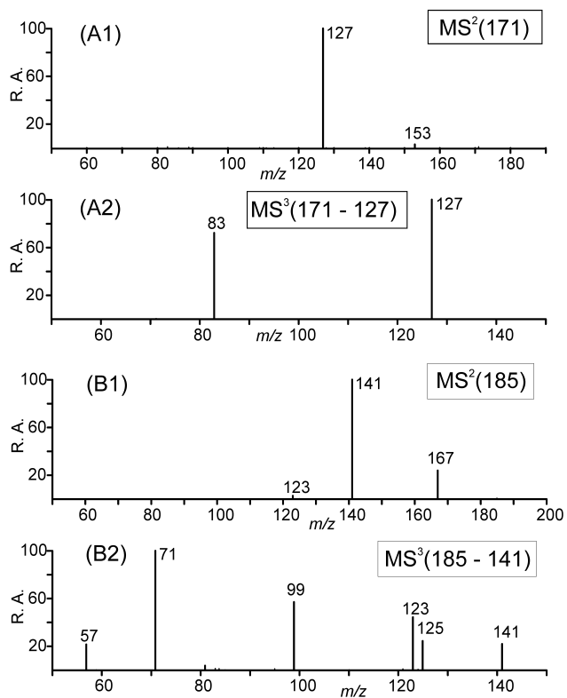
Fig. 3. (–)ESI-MS data for (A) terpenylic acid and (B) cis -pinic acid.
