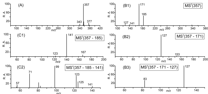
Fig. 4. (–)ESI-MS data for the major MW 358 compound (RT 24.7 min; Fig. 1a) present in \alpha -pinene ozonolysis SOA, assigned to a covalent dimer of the ester type: (A) first-order mass spectrum; (B1) m/z 357 MS^2 spectrum; (B2) and (B3) m/z 357 \rightarrow m/z 171 MS^n ( n = 3, 4 ) spectra; and, (C1) and (C2) m/z 357 \rightarrow m/z 185 MS^n ( n = 3, 4 ) spectra.
