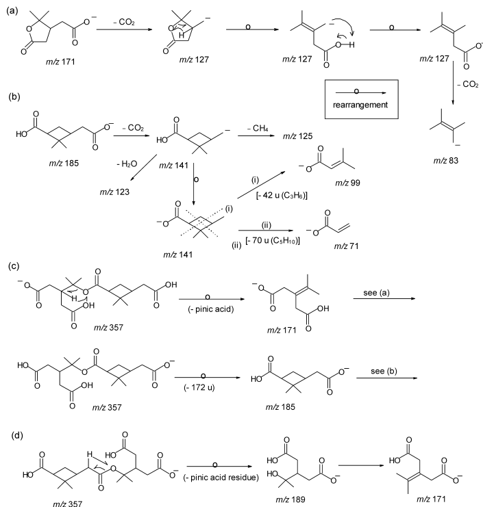
Scheme 1. Proposed fragmentation pathways for deprotonated (a) terpenylic acid, (b) cis -pinic acid, and the (c) major and (d) minor MW 358 compounds.
