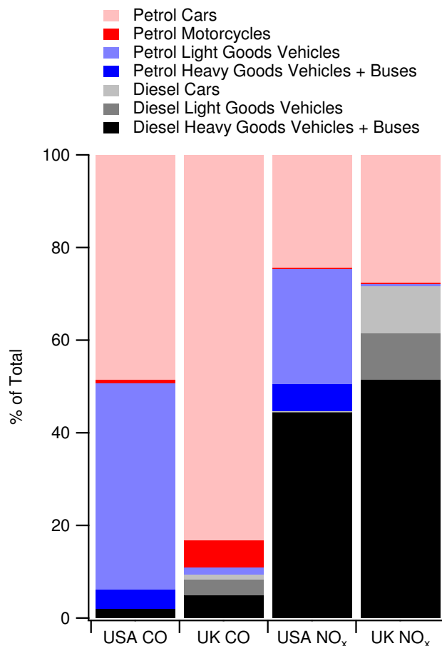
Fig. 8. Percentages of transport CO and NO_x for the USA and UK according to vehicle and fuel type. USA data is taken from the 2005 Environmental Protection Agency Atmospheric Emissions Inventory. UK data is taken from the 2006 Department of the Environment, Food and Rural Affairs National Atmospheric Emissions Inventory.
