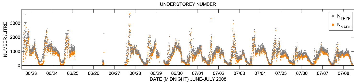
Figure S1 Number concentration of understorey particles deemed to be exhibiting NADH or Tryptophan-like fluorescence.
