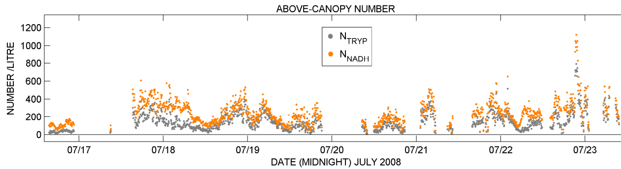
Figure S2 Number concentration of above-canopy particles deemed to be exhibiting NADH or Tryptophan-like fluorescence.
