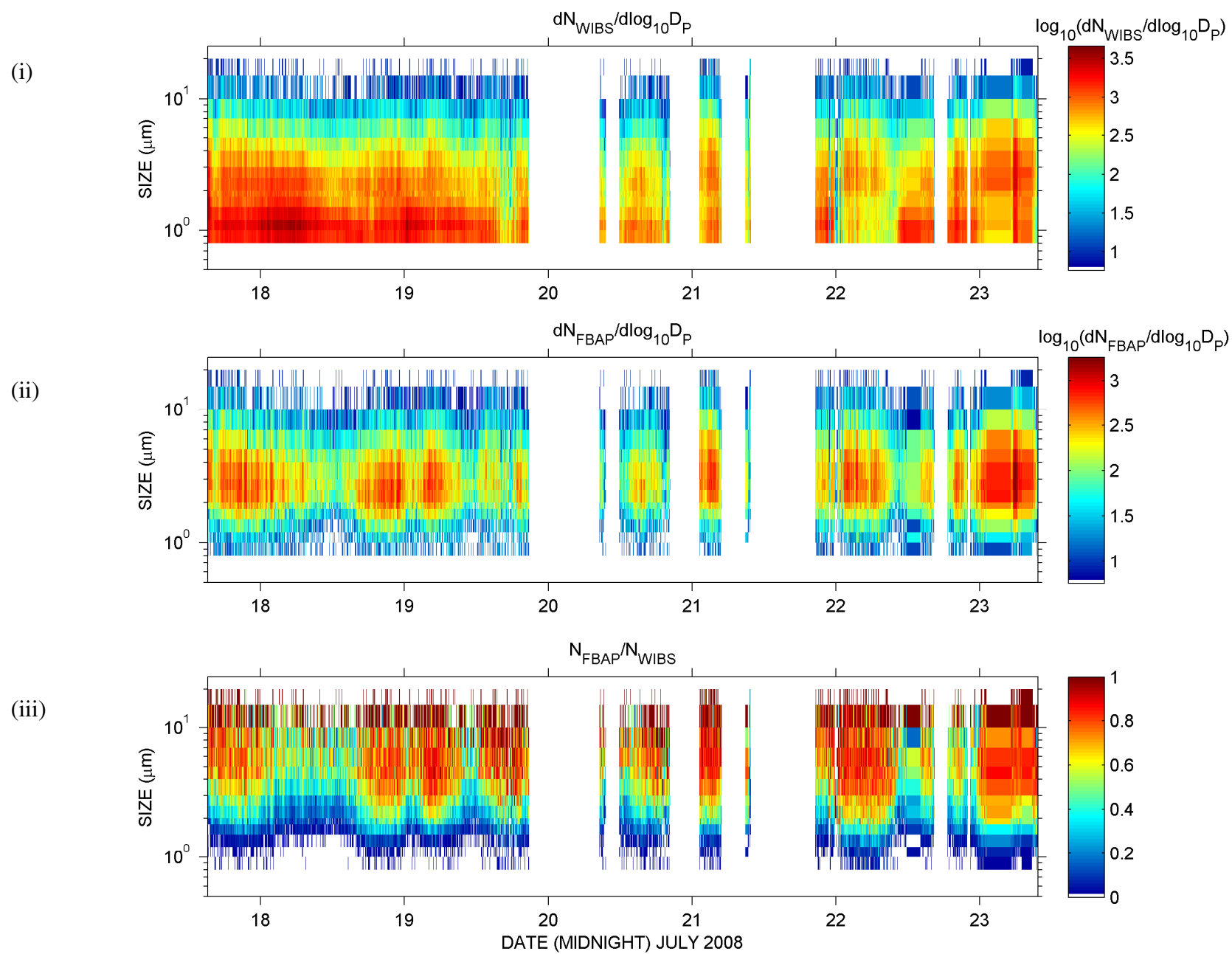
Figure S4 Time-resolved number size distributions of (i) N_{\text{WIBS}} , (ii) N_{\text{FBAP}} and (iii) the number fraction of N_{\text{FBAP}} above canopy, July 2008
