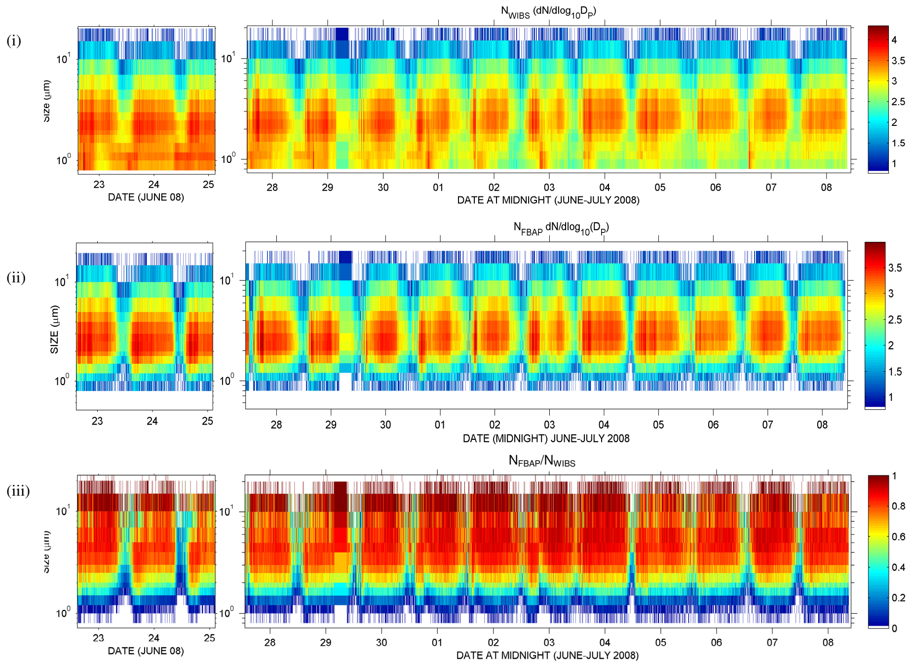
Figure S3 Time-resolved number size distributions of (i) N_{WIBS} , (ii) N_{FBAP} and (iii) the number fraction of N_{FBAP} in the understorey, June-July 2008
